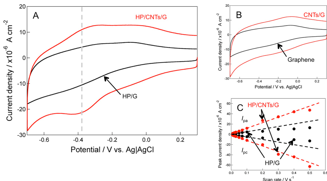
Figure 4. CVs of (A) HP/CNTs/G and HP/G and (B) CNTs/G and graphene electrodes in a 67 mM phosphate buffer solution (pH 7.4) at scan rate of 100 \text{mV s}^{-1} . (C) Relationship between anodic and cathodic peak currents of HP/CNTs/G and HP/G electrodes and scan rate.
