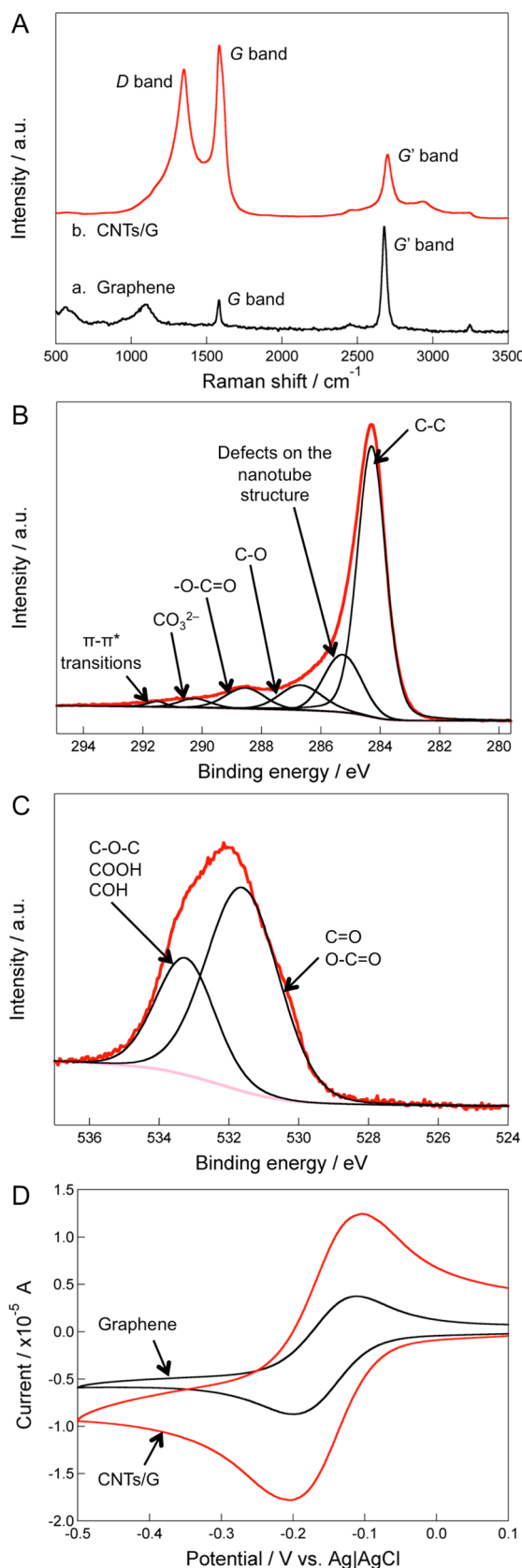
Figure 3. (A) Raman spectra of (a) graphene and (b) the CNTs/G film. XPS (B) C1s and (C) O1s spectra of the CNTs/G film. (D) CVs of 1.0 mM [\text{Ru}(\text{NH}_3)_6]\text{Cl}_3 in a 0.1 M KCl aqueous solution at the CNTs/G and graphene electrodes at a scan rate of 25 mV s -1 .
