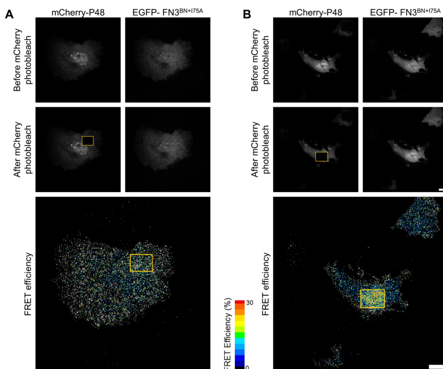
Figure 5. Performance of the P48 FREX sensor in mammalian cell cultures. Representative raw images of Cos-7 cells transfected with (A) EGFP-FN3 BN+I75A and mCherry-P48 and (B) EGFP-FN3 BN+I75A , mCherry-P48, and SH2. The top and middle rows show fluorescence before and after, respectively, the mCherry signal in the boxed area had been bleached. The FRET efficiency is plotted in the bottom row. The scale bar is 10 \mu m.
