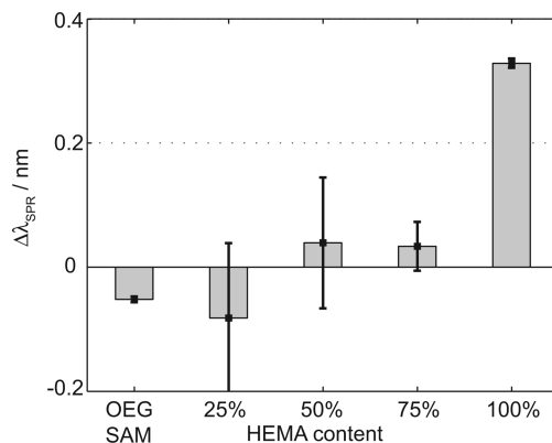
Figure 8. SPR response after deactivation of hydrogel matrix spot gradients with different HEMA content. The reading was made 2 min after a finished injection of 1.4 \mu\text{M} HFib dissolved in HBS-EP, pH 7.4. The confidence bars show the standard deviation from three spots on the same sample. For reference, the nonspecific binding to the HS-UDA-mPEG SAM is also shown. Only the response to the thickest hydrogel spots of each sample is shown (Note that the response level for 100% HEMA is close to the resolution of the imaging SPR instrument).
