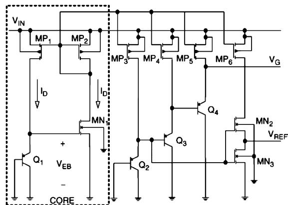
Figure 53. Proposed voltage reference circuit. Reprinted with permission from ref 76. Copyright 2012 IEEE.
