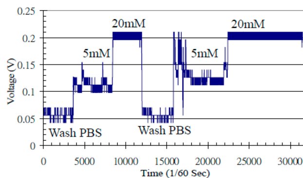
Figure 82. Real-time wireless continuous monitoring of the glucose reaction. Reprinted with permission from ref 115. Copyright 2005 IEEE.
