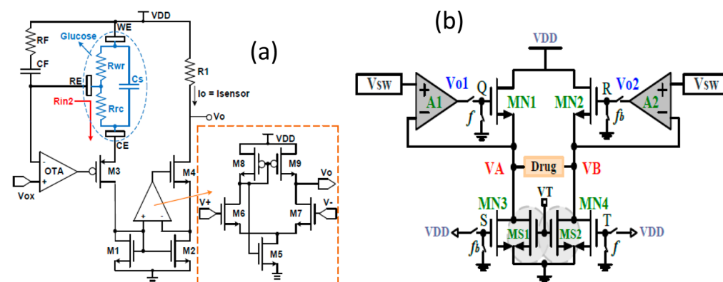
Figure 55. (a) Readout-2 (proposed wide-current-range potentiostat). (b) Core circuit of the drug driver. Reprinted with permission from ref 77. Copyright 2011 Taiwanese Society of Biomedical Engineering.
