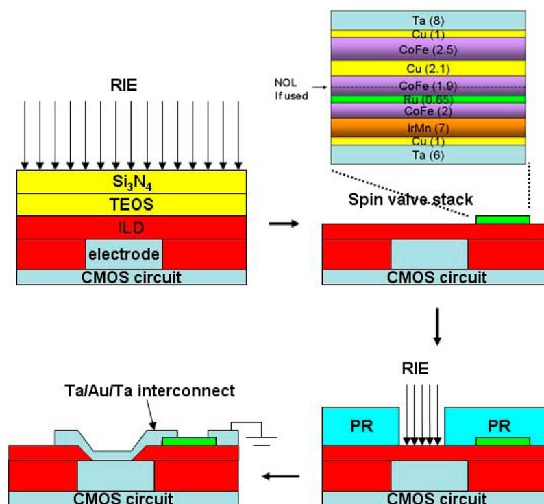
Figure 5. Micro- and nanofabrication steps for chip postprocessing. Reprinted with permission from ref 23. Copyright 2009 IEEE.
