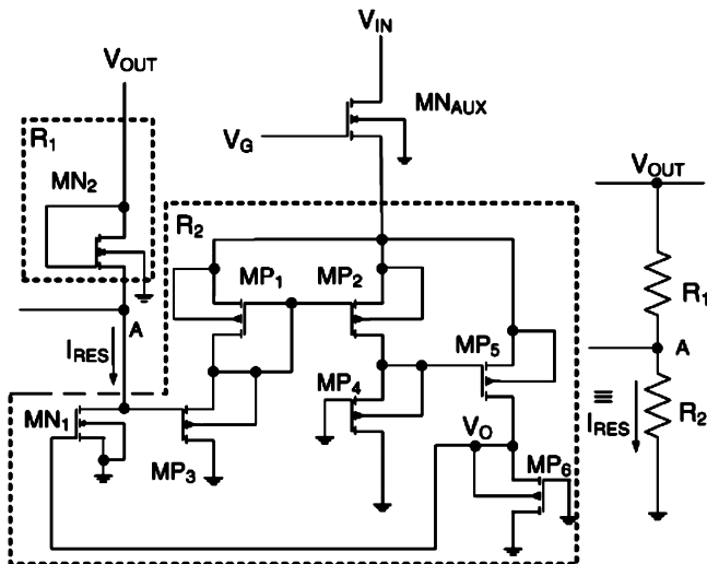
Figure 54. Sampler circuit. Reprinted with permission from ref 76. Copyright 2012 IEEE.
