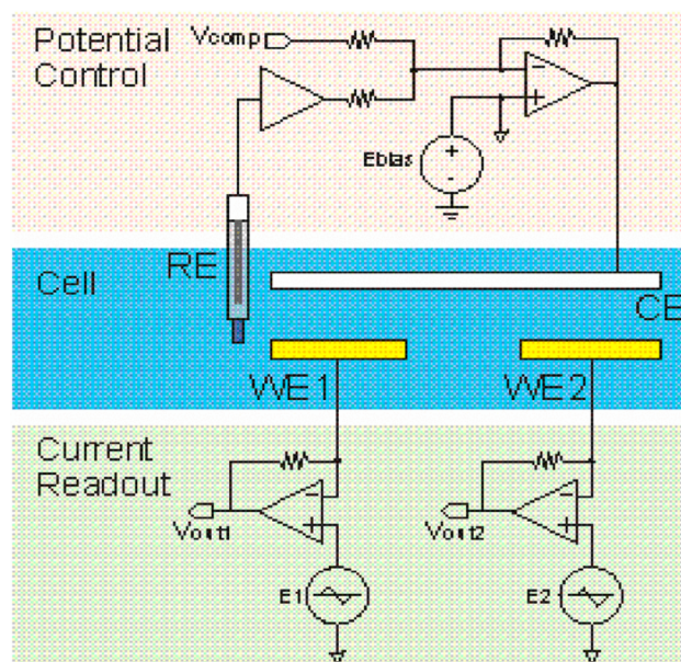
Figure 12. Architecture of the CMOS bipotentiostat with a connected counter electrode (CE), reference electrode (RE), and working electrodes (WEs). Reprinted with permission from ref 53. Copyright 2009 IEEE.
