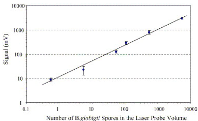
Figure 75. Quantitative determination of B. globigii spores. Fluorescence intensities were obtained as a result of the enzymatic reaction between the immunocomplexes and enzyme substrates. Reprinted with permission from ref 97. Copyright 2005 Elsevier.
