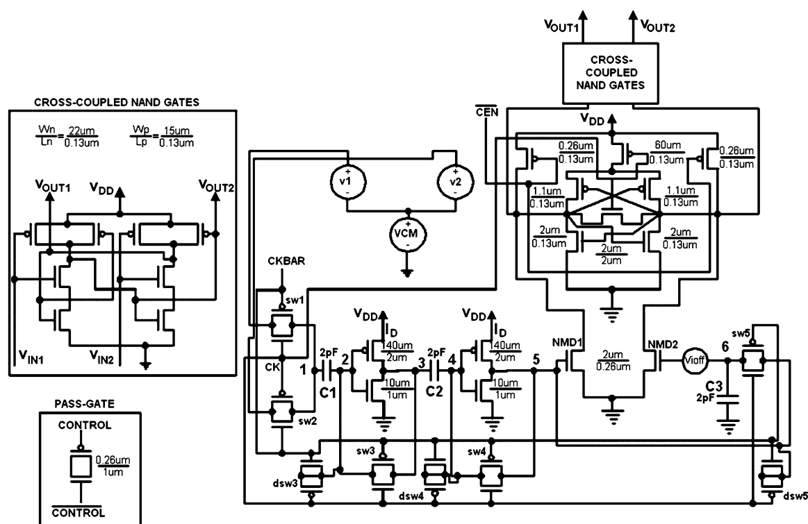
Figure 47. Complete CMOS circuit diagram of the proposed sampled data offset-compensated low-voltage comparator. Reprinted with permission from ref 74. Copyright 2008 Springer.
