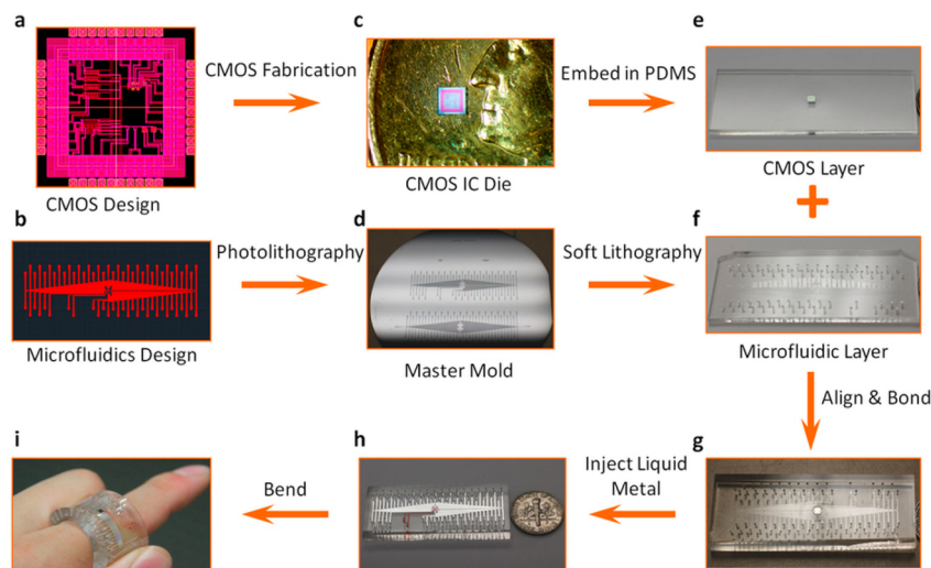
Figure 8. Schematic illustration of the fabrication and packaging procedures to produce flexible CMOS/microfluidic hybrid microsystems. Reprinted with permission from ref 35. Copyright 2013 Nature Group.
