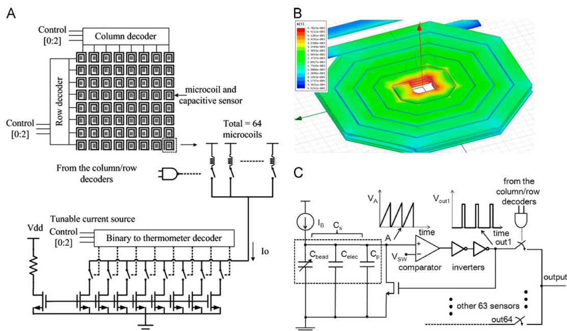
Figure 71. (a) Schematic of the CMOS micromanipulation and biosensing array. The tunable current source for driving microcoils is also illustrated. (b) Finite-element simulation of magnetic fields of the type-B microcoil. (c) Schematic of the capacitive sensing circuit. Reprinted with permission from ref 5. Copyright 2013 Elsevier.
