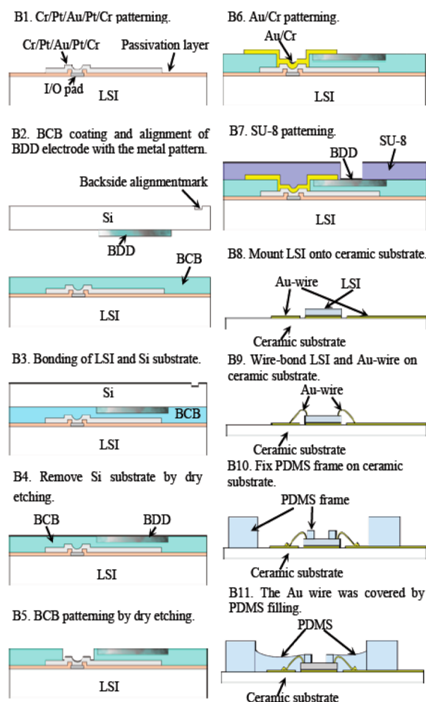
Figure 6. Fabrication process of a CMOS-based amperometric biosensor array with BDD electrodes. Reprinted with permission from ref 28. Copyright 2014 IEEE.
