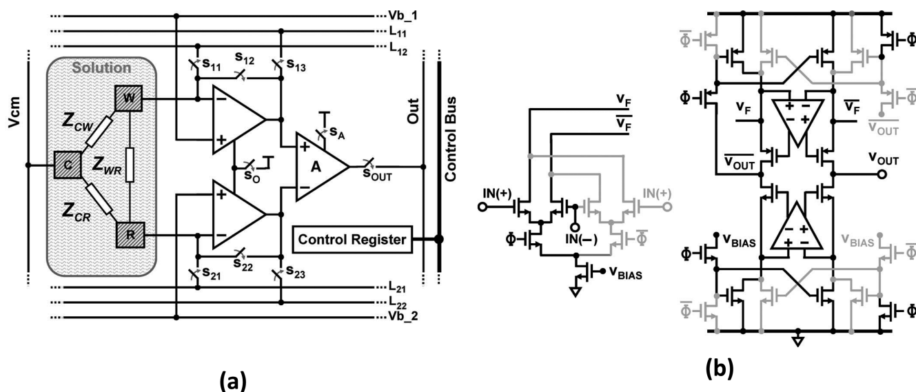
Figure 19. (a) Topology of the configurable sensor. (b) Opamp gain-boosted topology with switched biasing for low-frequency noise suppression. The gray paths indicate the alternative paths required for switched biasing. \Phi and \bar{\Phi} are the switching signals. Reprinted with permission from ref 43. Copyright 2006 IEEE.
