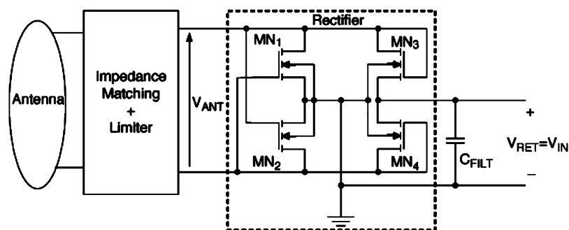
Figure 52. LVR front-end interface. Reprinted with permission from ref 76. Copyright 2012 IEEE.
