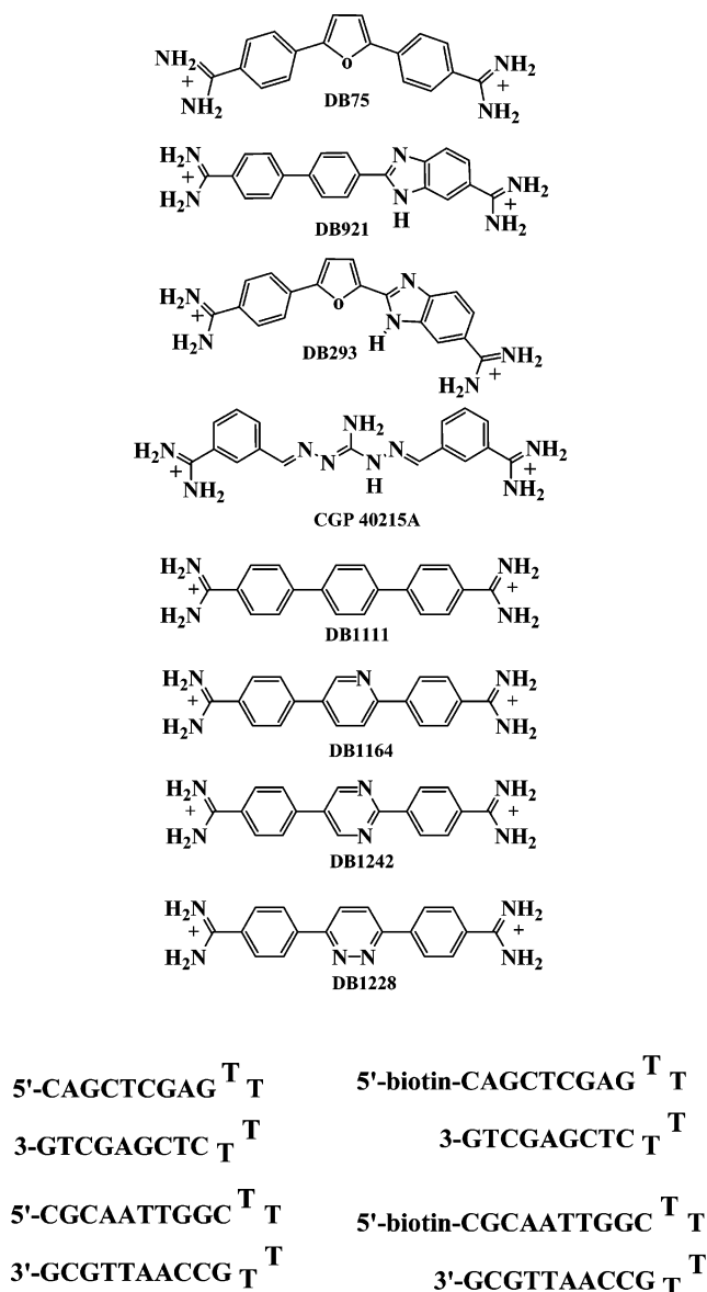
Figure 1. Compound structures and DNA oligomer sequences used in this study.
