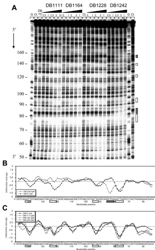
Figure 2. DNase I footprinting titration experiments. The pBS plasmid was isolated and purified from E. coli using Qiagen columns. The 265 bp DNA fragment was prepared by 3'-[ ^{32} P]-end labeling of the Eco RI- Pvu II double digest of the pBS plasmid (Stratagene) using \alpha -[ ^{32} P]-dATP and AMV reverse transcriptase. (A) The products of the DNase I digestion were resolved on an 8% polyacrylamide gel containing 8 M urea. Drug concentrations are at the top of the lanes. Tracks labeled G represent dimethylsulfate piperidine markers specific for guanines. Differential cleavage plots compare the susceptibility of the DNA to cutting by DNase I in the presence of (B) DB75 and DB1242, and (C) DB75, DB1111, DB1164, and DB1228. Deviation of points toward the lettered sequence (negative values) corresponds to a ligand-protected site, and deviation away (positive values) represents enhanced cleavage. The vertical scale is in units of \ln(f_a) - \ln(f_c) , where f_a is the fractional cleavage at any bond in the presence of the drug and f_c is the fractional cleavage of the same bond in the control.
