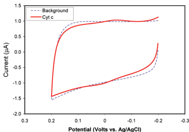
Figure 3. Cyclic voltammety of a \text{Zn}^{2+} -linked MUA MPC film with (solid line) and without (dashed line) adsorbed cyt c. The signal of the cyt c is obscured by the poorly compensated background signal. Voltammety was recorded at 100 mV/s in 4.4 mM potassium phosphate buffer (pH = 7).
