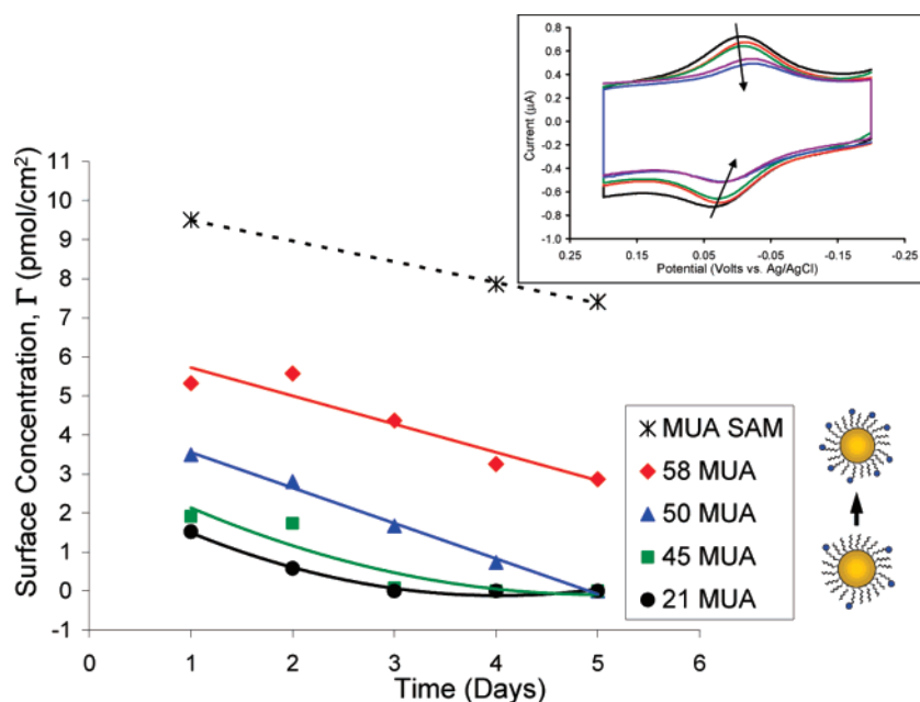
Figure 8. Surface concentration ( \Gamma ) of cyt c at dithiol-linked MPC film assemblies with varying MUA ligands in the final layer tracked over 5 days. Inset: Corresponding cyclic voltammetry of cyt c at a 58 MUA MPC film assembly showing denaturation of the protein (decreasing coverage) over time. Voltammetry was recorded at 100 mV/s in 4.4 mM potassium phosphate buffer (pH = 7).
