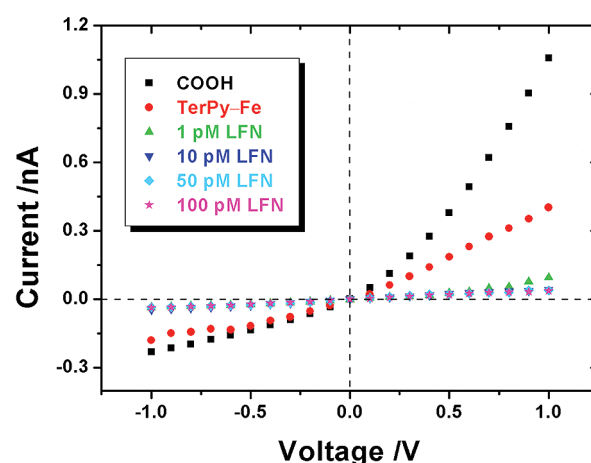
Figure 2. I – V characteristics of a single conical nanopore with tip d \approx 13 nm measured in 0.1 M KCl (pH 7.0) solution corresponding pore surface with carboxylate groups (black square), and iron–terpyridine complexes (red filled circle); and upon exposing the modified pore to different concentration of lactoferrin prepared (separately) in the same electrolyte solution, respectively.
