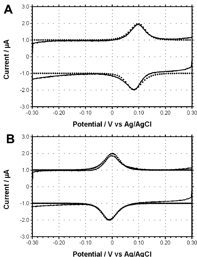
Figure 4. (A) Cyclic voltammograms of a mixed monolayer of \text{H}_2\text{Q} -OPE and PEG compared to the simulated CV (dotted line) on a gold coil working electrode. Simulation parameters: E_1 = 0.09 V vs Ag/AgCl, k_{e1} = 35 s ^{-1} , \alpha = 0.5 , \Gamma = 2 \times 10^{-12} mol/cm ^2 , capacitance = 5 \mu\text{F} , and electrode area = 1 cm ^2 . (B) Cyclic voltammograms after reaction with 1 \mu\text{M} mercaptoethanol compared to the simulated CV (dotted line). Simulation parameters: E_3 = -0.005 V vs Ag/AgCl, k_{e3} = 50 s ^{-1} . Coverage, capacitance, electrode area, and \alpha are the same as in (A).
