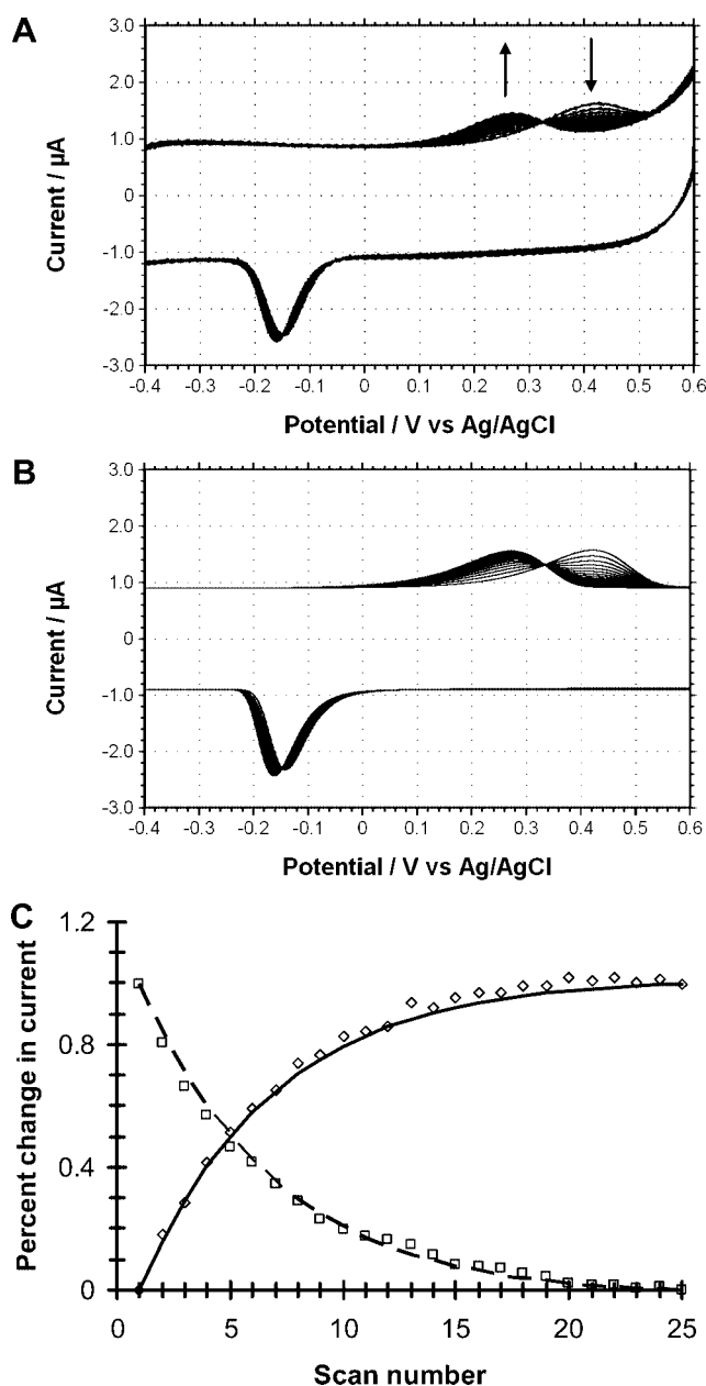
Figure 5. (A) Cyclic voltammograms of a mixed monolayer of \text{H}_2\text{Q} -alkane and PEG on a gold coil working electrode with the addition of 1 \mu\text{M} mercaptoethanol to the buffer. Scan rate = 200 mV/s. Number of scans = 25. (B) Simulated cyclic voltammograms using model 1 as described in the Experimental Section. Parameters: k_r = 0.038 s ^{-1} . All other parameters are the same as in Figure 1B. (C) Percent change of the anodic peak currents for the reactant ( \square ) and product ( \diamond ) vs scan number comparing the data with the simulation.
