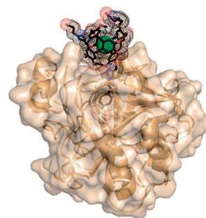
Figure 1. Crystal structure showing C8B –Xe–CAII interactions. 29 The Xe atom (green) is shown with a van der Waals diameter of 4.3 Å, the \text{Zn}^{2+} ion is gray, the CAII backbone and surface are tan, and the \text{M}_6\text{M}_6 enantiomer of C8B is shown in black (carbon), red (oxygen), and blue (nitrogen), surrounded by its van der Waals surface (dots). C8B binds in the active site with the sulfonamide anion coordinated to \text{Zn}^{2+} .
