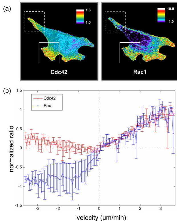
Figure 4. Migrating MEF cells containing both a FRET-based Rac1 biosensor and CRIB199 , a Cdc42 biosensor based on mero199 conjugated to the CRIB domain of WASP. (a) Ratiometric images of Cdc42 and Rac1 activity (dotted box = cell tail undergoing retraction, solid box = protrusion along the leading edge). Note that the leading edge protrusion in the box shows high
