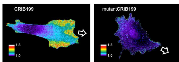
20 21 22 23 24 25 26 27 28 Figure 3. Migrating MEF cells microinjected with CRIB199 , the biosensor based on mero199 29 conjugated to the CRIB domain, show Cdc42 activity in protrusions at the leading edge. Cells 30 containing a mutant biosensor with reduced affinity for Cdc42 (mutant CRIB199 ) showed 31 substantially less Cdc42 activation (images are scaled identically to show this). The pseudocolor 32 scale shows the increase in ratio relative to the lowest 5% of ratio values in the cell (see Figure 33 S5). These low values were similar for the two biosensors. The white arrow indicates the 34 direction of movement. 35 36 37 38 39 40 41 42 43 44 45
