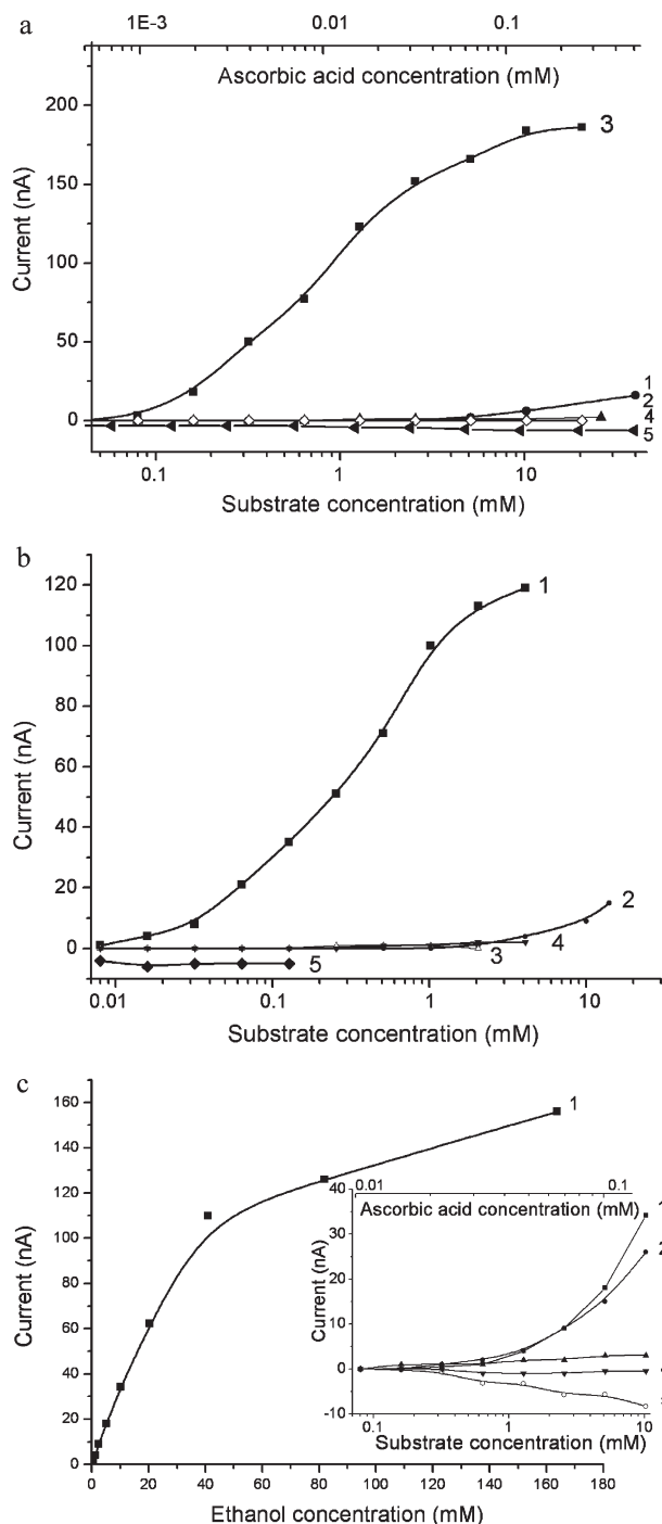
Figure 3. Responses of lactate (a), glucose (b), and ethanol (c) biosensors to 1, ethanol; 2, glycerol; 3, glucose; 4, lactate; and 5, ascorbic acid. Measuring conditions: 20 mM phosphate buffer at pH 7.2, at a potential of +200 mV versus the intrinsic reference electrode.
