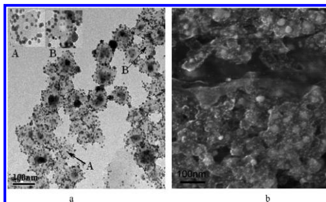
Figure 2. TEM (a) and SEM (b) of AuNPs-AgCl@PANI. The insets in (a) show the enlarged view of the regions arrows A and B pointed.
