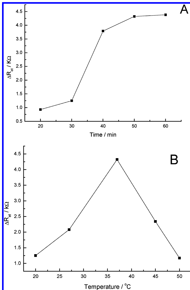
Figure 8. Relationships of \Delta R_{\text{et}} with the incubation time (A) and incubation temperature (B). Faradaic impedance spectra were obtained in PBS (pH 7.0) containing 2 mM [\text{Fe}(\text{CN})_6]^{3-/4-} .
