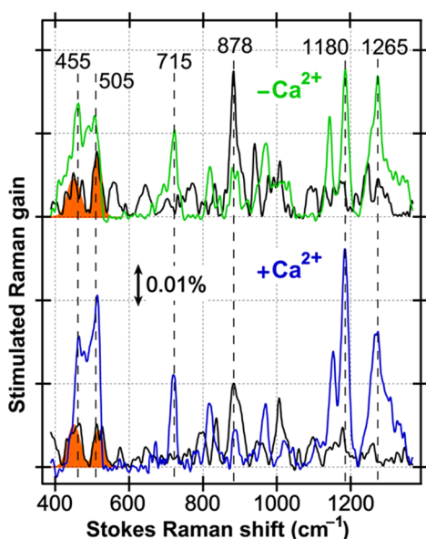
Figure 2. Comparison of the ground-state and T = 0 fs excited-state FSRS spectra of the \text{Ca}^{2+} -free and bound GEM-GECO1. For the \text{Ca}^{2+} -free protein, the S_0 spectrum (black solid trace, upper panel) is overlaid with the S_1 spectrum at photoexcitation time zero (green solid trace). For the \text{Ca}^{2+} -bound protein in the lower panel, the S_0 and S_1 ( T = 0 fs) spectra at time zero are shown by the black and blue solid traces, respectively. Two marker bands below 600\text{ cm}^{-1} are shaded with orange Gaussian-fitted peaks in S_0 , which are greatly enhanced in S_1 . Prominent vibrational modes are indicated by vertical dashed lines with their frequencies labeled above. The double-headed black vertical line represents the absolute stimulated Raman gain strength of 0.01%. A rearranged version of this figure that directly overlays the two S_0 spectra ( \text{Ca}^{2+} free versus bound) and two S_1 spectra at T = 0 fs ( \text{Ca}^{2+} free versus bound) for comparison is shown in Figure S4 in the Supporting Information.
