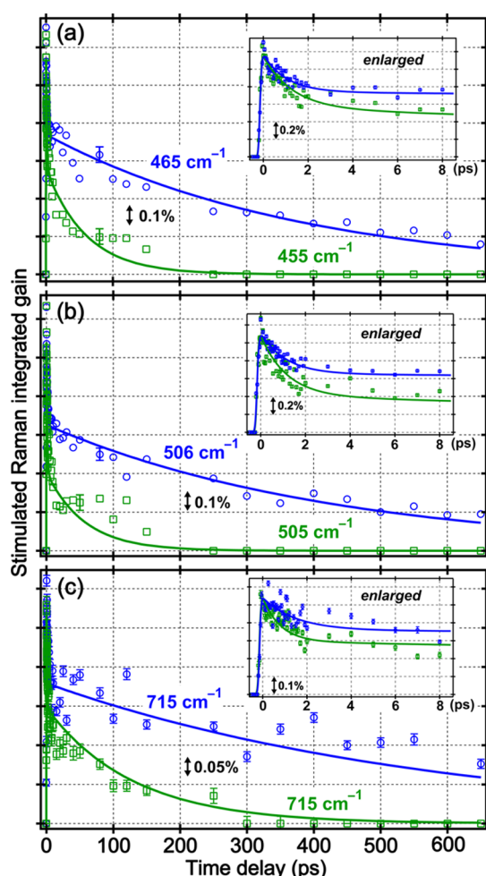
Figure 4. Time evolution of three relatively low frequency excited-state Raman modes in the \text{Ca}^{2+} -free and bound GEM-GECO1 shows distinct patterns. Intensity kinetic plots of modes at (a) 455 and 465 \text{cm}^{-1} , (b) 505 and 506 \text{cm}^{-1} , and (c) 715 and 715 \text{cm}^{-1} for the \text{Ca}^{2+} -free (green) and bound (blue) proteins, respectively, in aqueous buffer solution following 400 nm photoexcitation up to 650 ps. All the modes in both protein samples show double exponential decay (fits are shown in solid lines, and the experimental time zero retrieved from least-squares fitting is ca. -150 fs), but the second decay time for the \text{Ca}^{2+} -bound protein is much longer than that for the \text{Ca}^{2+} -free protein. The enlarged dynamics plot within 8 ps exhibits a similar initial relaxation phase ( <2 ps decay time constant, see Table 1), regardless of \text{Ca}^{2+} binding (shown in the insets). The typical error bars (one standard deviation of the Gaussian-fitted peak area, at least three independent data sets) are shown for one time delay point in (a) and (b) and for all the data points in (c) where the peak intensity is weaker. The absolute magnitude of the Raman integrated gain is noted in each subfigure as the vertical double-headed line. The apparent larger spread of data points in the inset of (c) is due to mode intensity quantum beating (Figure S6) on the sub-ps to ps time scale.
