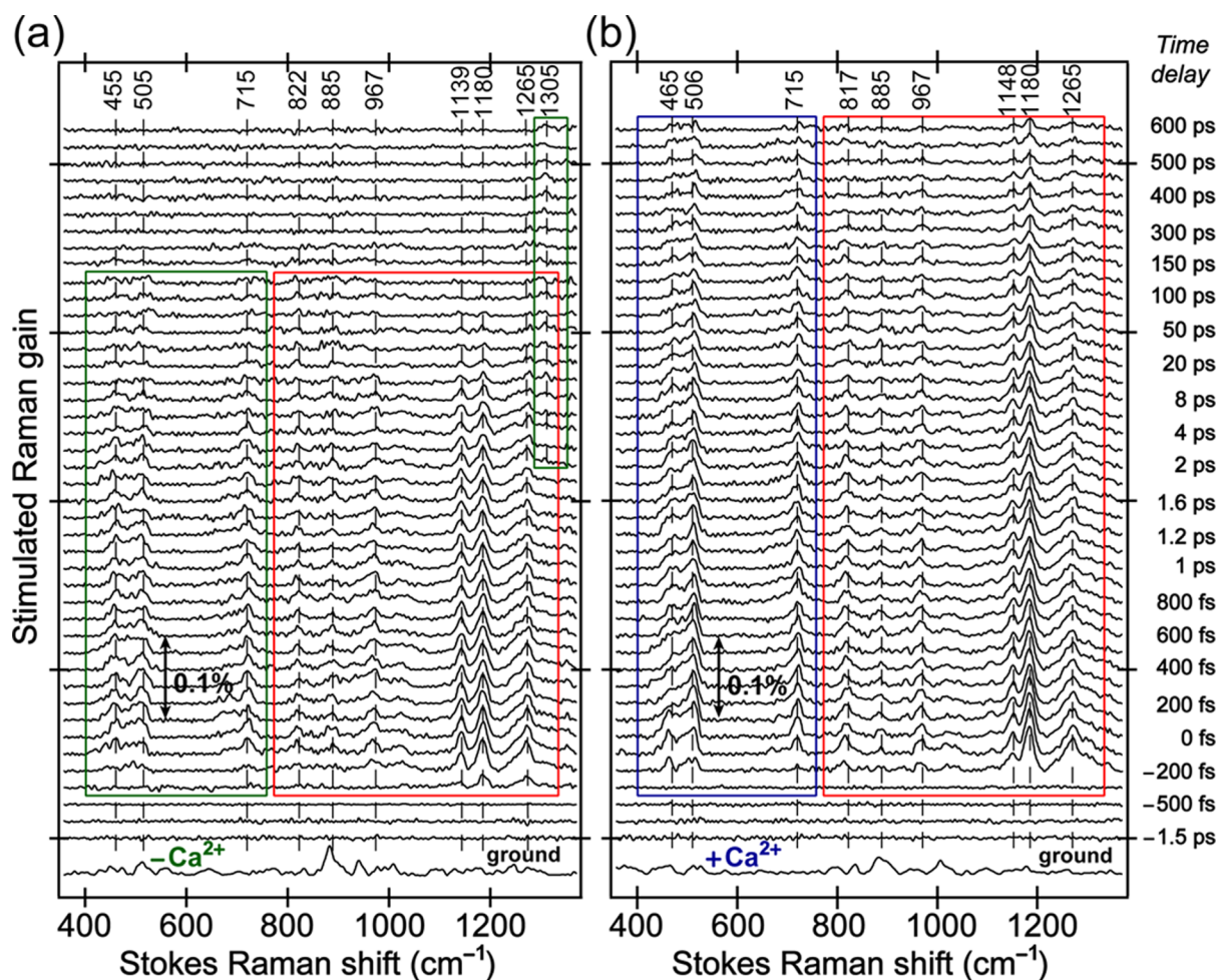
Figure 3. Time-resolved excited-state FSRS spectra of both (a) Ca 2+ -free and (b) Ca 2+ -bound GEM-GECl1 from -1.5 to 600 ps following 400 nm photoexcitation. The Raman pump is centered at 802 nm. The buffer-removed ground-state FSRS spectra of the proteins are plotted at the bottom for comparison within a spectral window of about 350–1400 cm -1 . Every other time delay between the fs photoexcitation and Raman probe pulses is labeled on the right side of the spectra. Not all the time points are shown. The two red boxes enclose the high-frequency (>800 cm -1 ) modes, while the large green/blue box in the Ca 2+ -free/bound spectra emphasizes the lower frequency modes. The small green rectangle in the upper right corner of (a) highlights the 1305 cm -1 mode of I* in the Ca 2+ -free protein. The center frequency of the prominent S_1 modes throughout the detection time window is labeled on the top. The absolute Raman gain strength of 0.1% is shown with the double-headed arrow.
