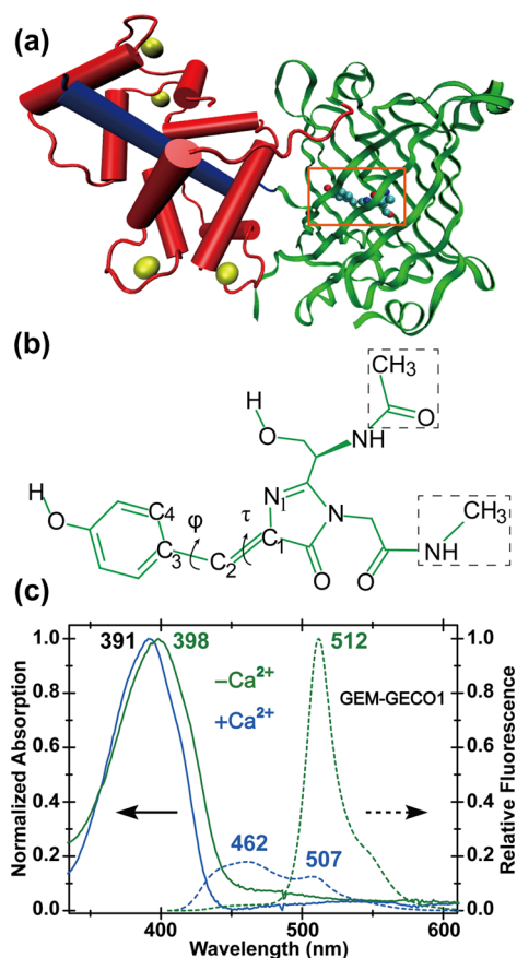
Figure 1. Illustrative structure of the GEM-GECO1 biosensor for \text{Ca}^{2+} imaging and its electronic spectroscopy results. (a) Protein structure of GEM-GECO1 in the \text{Ca}^{2+} -bound state, as represented by the analogous GCaMP2 (PDB ID 3EVR), 36 with the circularly permuted GFP (cpGFP) \beta -barrel in green, the CaM domain in red, the M13 peptide in blue, and the calcium ions bound to CaM in yellow. The structure is rendered using VMD. 66 The embedded chromophore near the \beta -barrel opening is indicated by the orange box. (b) Molecular structure of the SYG chromophore. The methyl group of Thr223 is replaced by an H atom without further structural modification to obtain the SYG chromophore. The connections to the protein backbone are capped with \text{CH}_3\text{CO} at the N terminus and \text{NHCH}_3 at the C terminus, respectively. The \tau ( \text{N}_1\text{--C}_1\text{=C}_2\text{--C}_3 ) and \phi ( \text{C}_1\text{=C}_2\text{--C}_3\text{--C}_4 ) dihedral angles are also shown. (c) Normalized UV/Vis absorption spectra of the \text{Ca}^{2+} -free (green solid curve, left axis) and \text{Ca}^{2+} -bound (blue solid curve) GEM-GECO1. The steady-state relative emission spectra of GEM-GECO1 ( \lambda_{\text{ex}} = 400 nm) in the absence (green dashed curve, right axis) and presence (blue dashed curve) of \text{Ca}^{2+} show dramatic differences.
