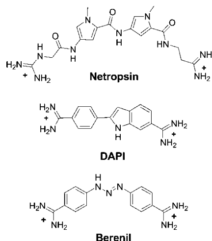
Figure 1. Chemical structures of three dicationic minor-groove binding compounds.
