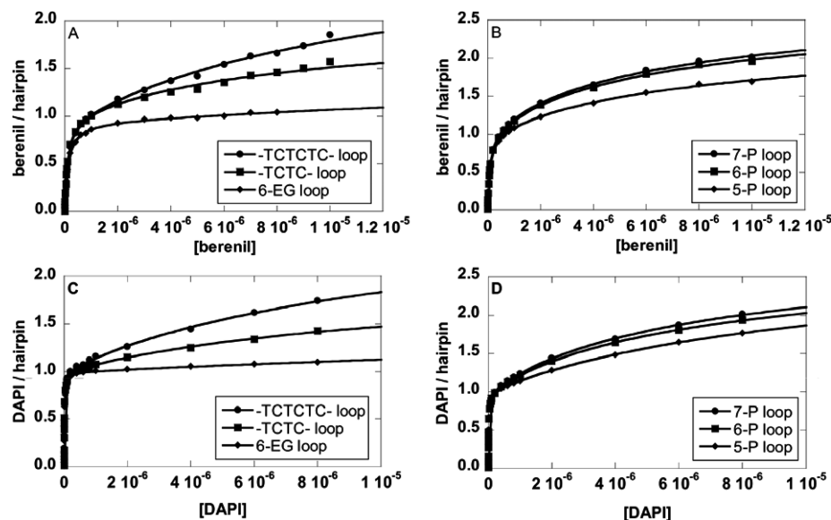
Figure 5. Binding isotherms of berenil to an 8-bp stem DNA hairpin with 6-EG, TCTC, or TCTCTC loop (A), with a 5-P, 6-P, or 7-P loop (B); and of DAPI (C and D) to the same hairpins. Salt concentrations were 92 mM NaCl and 192 mM NaCl for berenil and DAPI, respectively.
