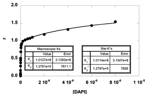
Figure 7. Fittings of the SPR binding results of DAPI with an 8-bp stem DNA hairpin containing a TCTC loop. The data were fitted with a two-site model using eq 1 or eq 2. The two fitting curves overlap on top of each other, and the fitted parameters illustrate the relationship: K_1 = (K_1^* + K_2^*) and K_2 = (K_1^* K_2^*) / (K_1^* + K_2^*) . The macroscopic binding constants are practically the same as the site binding constants ( K_1 = K_1^* ). This is expected since K_1^* is much greater than K_2^* .
