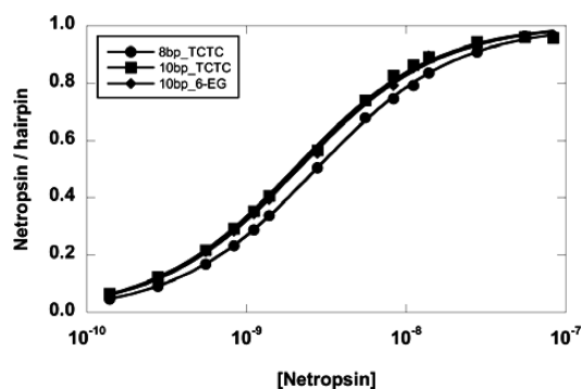
Figure 6. Binding isotherms of netropsin to three DNA hairpins. The primary binding affinity to a short 8-base-pair stem with a TCTC loop (5'-CGAATTCGTCTCCGAATTCG-3' or 8bp_TCTC) is lower than that of a 10-base-pair stem with the same loop (5'-GCGAATTCGCTCTCGCGAATTCGC-3' or 10bp_TCTC) or a 10-base-pair stem with a hexaethylene glycol loop (5'-GCGAATTCGCP(O) 3 (C 2 H 4 O) 6 GCGAATTCGC-3' or 10bp_6-EG).
