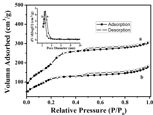
Figure 3. The nitrogen adsorption–desorption isotherms of (a) MMS and (b) Ru(bpy) 2 phen-MMS. The inset shows the pore size distribution curve of (a) MMS and (b) Ru(bpy) 2 phen-MMS.
