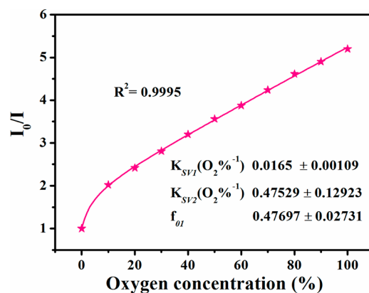
Figure 7. Typical luminescence-intensity-based Stern–Volmer plot for Ru(bpy) 2 phen-MMS.
