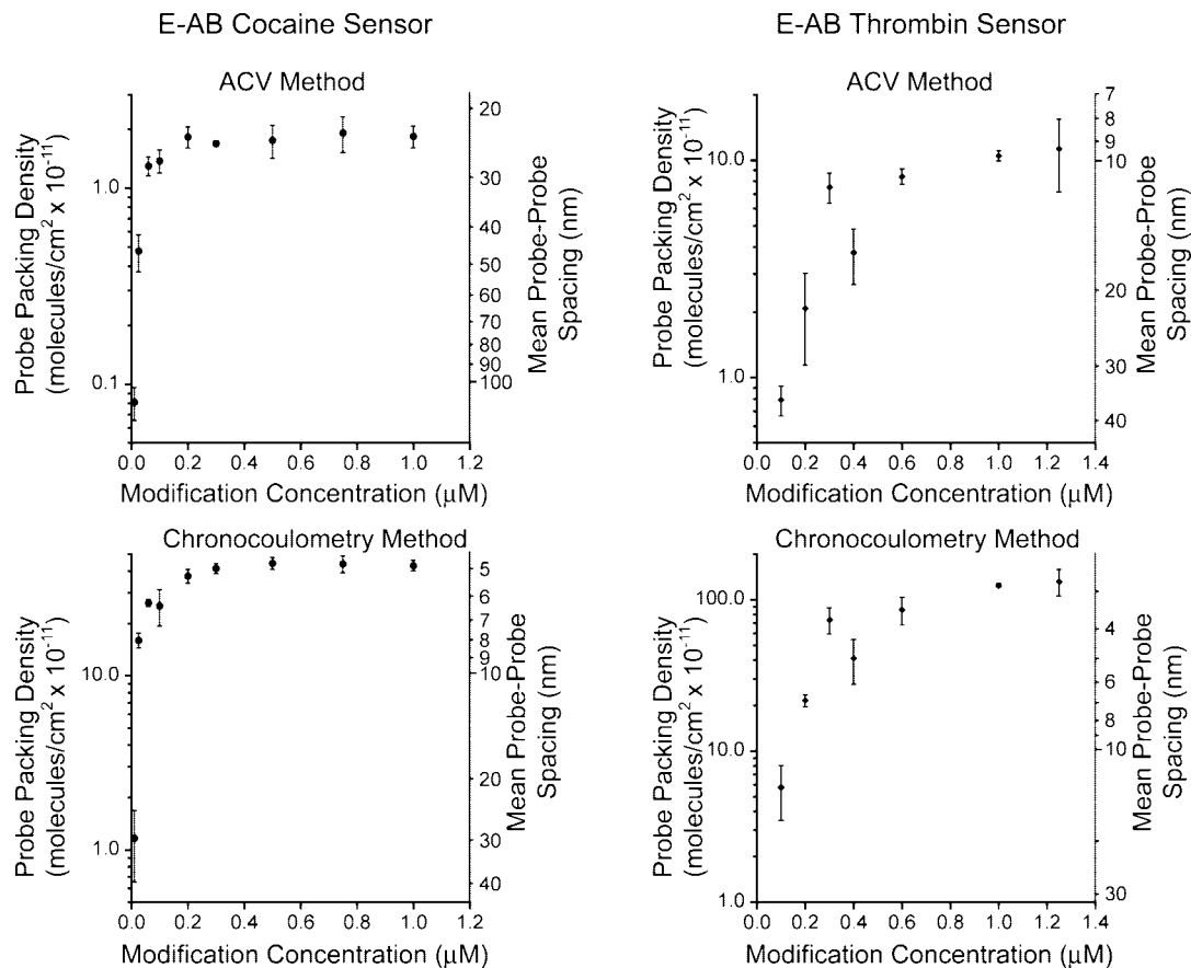
Figure 2. Packing density of aptamers on the electrode surface is readily controlled by varying the concentration of probe DNA employed during sensor fabrication. As shown, ACV peak current (top) and chronocoulometry (bottom) methods produce correlated, but significant different estimates of probe density. We believe this occurs because the AC method is highly dependent on electron transfer efficiency, which in turn is dependent on probe geometry. We have thus reported chronocoulometric measurements throughout the body of this work. Values represent the average and standard deviations from three independent sensors at each probe density.
