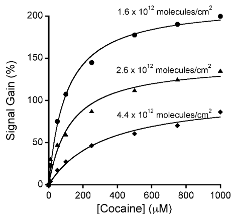
Figure 3. Density with which probe aptamers are packed on the electrode strongly affects E-AB signal gain. For example, shown are the response curves of low medium and high-density cocaine sensors (fabricated using 25, 60, and 500 nM cocaine aptamer concentrations during fabrication). The solid lines represent hyperbolic binding curves with dissociation constants ( K_d ) of 327 \pm 64 , 101 \pm 8 and 127 \pm 35 \mu M respectively, which are comparable to the solution phase aptamer K_d of 100 \mu M. 23
