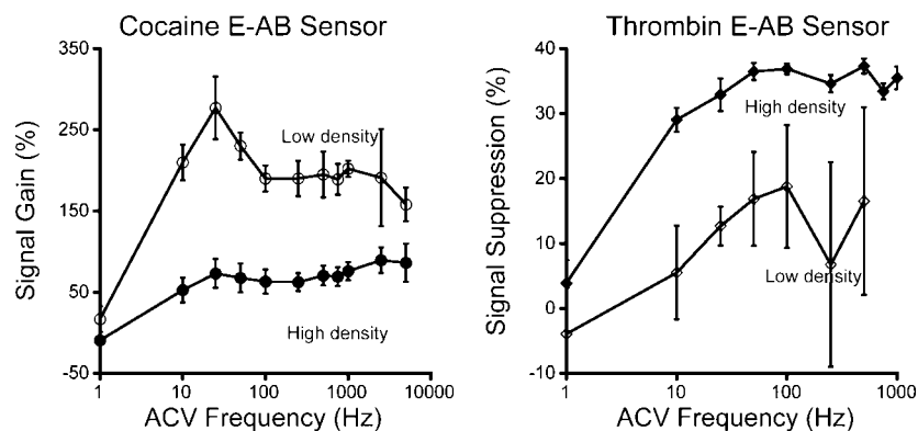
Figure 5. At all but the very lowest frequencies, E-AB signaling is relatively unaffected by the ACV perturbation frequency used to interrogate the surface bound aptamers. This effect holds for both the cocaine (left) and thrombin (right) sensors and for both low (open circles) and high (filled circles) packing densities. Shown are data collected with low ( 1.6 \times 10^{12} molecules/cm 2 ) and high ( 4.3 \times 10^{12} molecules/cm 2 ) density cocaine sensors and low ( 5.8 \times 10^{11} molecules/cm 2 ) and high ( 1.3 \times 10^{13} molecules/cm 2 ) density thrombin sensors.
