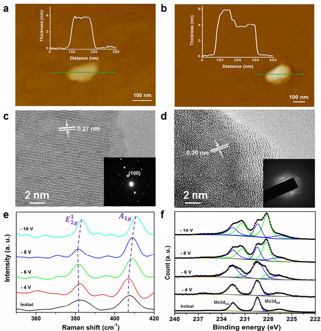
Figure 1. AFM and HRTEM images of flakes before and after the intercalation via a -10 V applied voltage are shown in (a) to (d). Examples of the AFM images and profiles for a 2D \text{MoS}_2 nanoflake (a) and a 2D \text{Li}_x\text{MoS}_2 nanoflake (b). (c) A HRTEM image of a pristine 2D \text{MoS}_2 nanoflake and its corresponding SAED pattern (inset). (d) A HRTEM image of an intercalated 2D nanoflake and its corresponding SAED pattern (inset). (e) Raman spectra of 2D \text{MoS}_2 and the spectra changes after \text{Li}^+ ion intercalation at different applied voltages. (f) XPS spectra of elemental Mo after \text{Li}^+ ion intercalation at different applied voltages (all XPS spectra are calibrated by a carbon 1s peak located at 284.50 eV). It is also noticed that a small peak appears at 236.0 eV, corresponding to \text{Mo}^{6+} 3d_{5/2} , which is a common characteristic for \text{Li}^+ intercalated \text{MoS}_2 , possibly due to the oxidation of a very small portion of \text{MoS}_2 .
