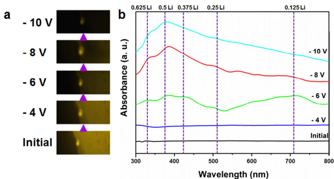
Figure 3. (a) PL images of films made of drop-casted 2D MoS 2 in initial and at the intercalating voltages of -4, -6, -8 and -10 V (at a broadband excitation light source covering wavelengths ranging from 400 to 500 nm.) The changes in PL of 2D nanoflakes at different applied voltages are presented. Yellow colored light is emitted from the 2D MoS 2 nanoflakes at the initial stage. When a voltage of -4 V is applied to the sample, the PL level is only slightly reduced. When the applied voltage is decreased from -6 to -10 V, PL intensity drops dramatically and there is a near total photo-quenching at the voltage of -10 V. (b) UV-Vis absorbance spectra of the 2D nanoflakes under different electrochemical forces, in which the pristine 2D MoS 2 is used as the differential reference. Main absorption peaks in the experimental are observed at 332, 380, 430, 498 and 714 nm. The wavelengths for theoretical estimates of plasmonic peaks as a function of intercalated Li + ions are listed along dot lines. An intercalated fluoride-doped tin oxide (FTO) peak is observed at 325 nm, showing a minimal interference (Figure S3 and Supporting Information Section S7).
