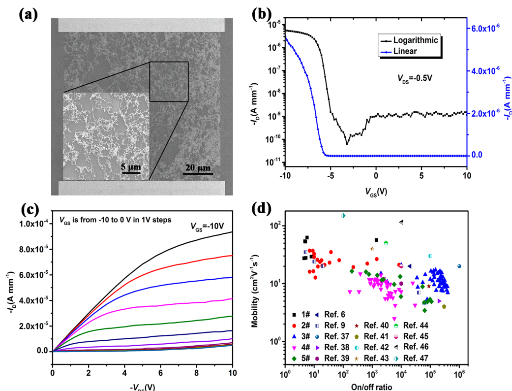
Figure 4. (a) Typical SEM image of the s-SWCNT thin film deposited on a Si substrate. (b) Typical transfer ( I_D – V_{GS} ) characteristic at V_{DS} of -0.5 V. (c) Output ( I_D – V_{DS} ) characteristics of the same device at various V_{GS} values ranging from -10 to 0 V. (d) Statistics of the carrier mobilities and on/off ratios of the TFTs fabricated using our 1#, 2#, 3#, 4# and 5# samples in comparison with those reported previously.
