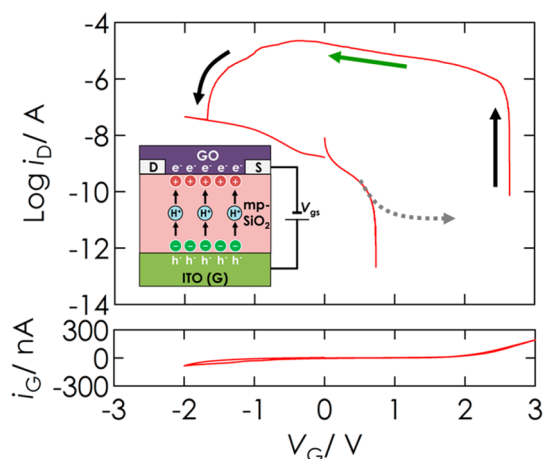
Figure 2. Electrical conduction characteristics of GO-based EDLT (schematically shown in inset) measured in air: i_D vs V_G (upper panel) and i_G vs V_G (lower panel). Sweep rate of V_G was 4 mV/s; V_D was 0.5 V.
