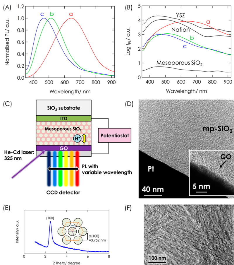
Figure 1. (A) Normalized PL spectra of three types of GO with different oxidation extents. Curves a, b, and c represent pristine GO, GO reduced by exposure to hydrazine vapor for 3 min, and GO reduced by exposure to hydrazine vapor for 10 min, respectively. (B) PL spectra of three proton-conducting solid electrolyte thin films (YSZ, Nafion, and mesoporous SiO 2 ). Three spectra in Figure 1A are also shown for comparison. (C) Schematic illustration of all-solid-state PL source made of GO and mesoporous SiO 2 thin film. (D) HR-TEM image of mesoporous SiO 2 (mp-SiO 2 )/GO/Pt interface. Inset shows magnification of GO layers. (E) The XRD pattern of mesoporous SiO 2 thin film. (F) FE-SEM image of mesoporous SiO 2 thin film in surface view.
