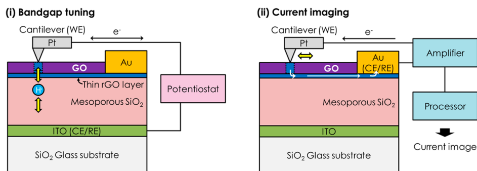
Figure 5. Schematic illustration of CAFM setups for bandgap tuning (i) and current imaging (ii). Thin rGO layer was inserted for current imaging (see Methods for details).
