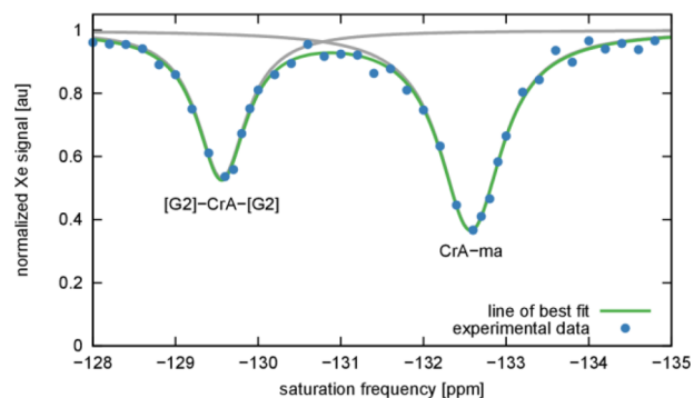
Figure 2. Hyper-CEST spectroscopy of [G2]-CrA-[G2] and CrA-ma in water +0.01% Antifoam A (Sigma) and 0.27% DMSO. Both xenon hosts are at an approximate concentration of 13 \mu M. The saturation frequency is relative to the frequency of free xenon in solution at 0 ppm. The data was fit using a negative exponential of the sum of two Lorentzians 14 (green lines, see the Supporting Information for more details). The contribution from each of the individual Lorentzians is shown with a grey line.
