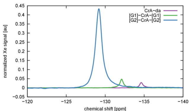
Figure 1. Direct Xe NMR of xenon hosts. Purple: saturated solution of CrA-da (peak at −134.6 ppm). Green: saturated solution of first generation construct [G1]-CrA-[G1] (peak at −132.1). Blue: 890 \mu M solution of second generation construct [G2]-CrA-[G2] (peak at −129.2). All samples in water +0.01% Antifoam A (Sigma). Spectra were averaged 32 times and are normalized and referenced to the signal from xenon free in solution (intensity 1 at 0 ppm). Each successive generation shifted the Xe@ cage resonance approximately 2.5 ppm toward the resonance of Xe free in solution. The first-generation construct only marginally increased the solubility of the CrA, while the second-generation construct was freely soluble in water.
