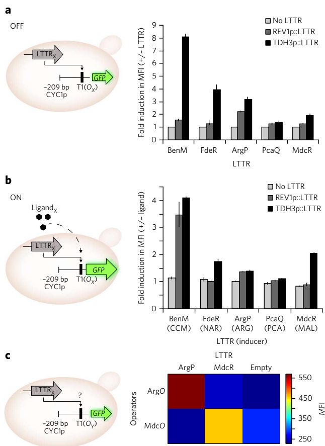
Figure 4 | Application of transcriptional activators from the LTTR family as biosensors in yeast. (a) Illustration of LTTR-mediated activation of GFP expression by binding to the cognate operator in position T1 of 209bp_CYC1p (left). The 209bp_CYC1p_T1 reporter promoter design supports GFP expression when controlled by individual LTTR transcriptional activators expressed from either a weak (REV1p) or a strong (TDH3p) promoter (right). The y axis shows fold induction in mean fluorescence intensity (MFI) in cells expressing individual LTTRs relative to cells not expressing the LTTRs. (b) Illustration on external application of individual ligands for induction of LTTR-mediated activation of GFP expression (left). External application of individual ligands can induce LTTR-mediated activation of GFP expression (right). The y axis shows fold induction in MFI for cells grown for 24 h in medium containing either CCM, naringenin (NAR), L-arginine (ARG), protocatechuic acid (PCA) or malonic acid (MAL) compared to cells growing in control medium. (c) Heatmap showing orthogonality of MdcR- and ArgP-mediated transcriptional regulation of GFP expression controlled by either reporter promoter 209bp_CYC1p_MdcO_T1 or 209bp_CYC1p_ArgO_T1 (Supplementary Table 4). Color key shows MFI from three ( n = 3 ) biological replicate experiments. For a and b , MFI values and their error bars are shown as mean \pm s.d. from three ( n = 3 ) biological replicates.
