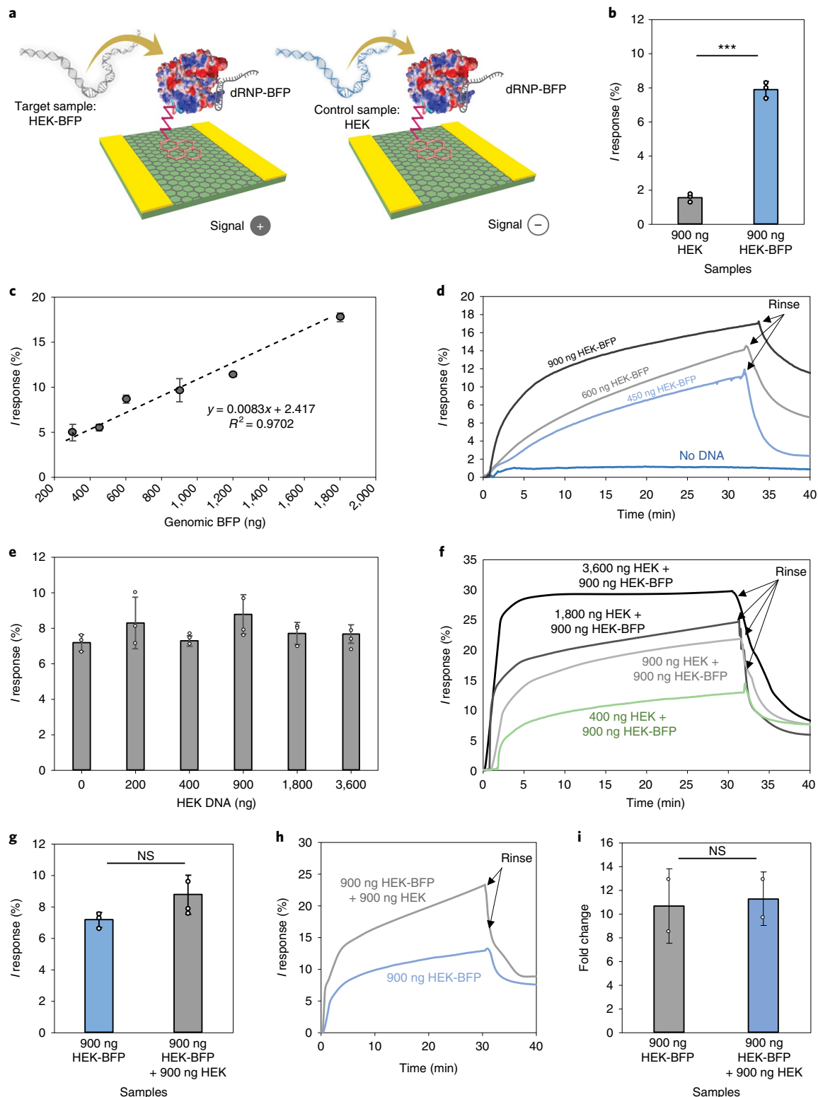
Fig. 5 | CRISPR-Chip sensitivity and selectivity of the bfp target contained within whole genomic samples. a , Solutions of HEK-BFP (left) and HEK DNA (right) were analysed with the dRNP-BFP-functionalized CRISPR-Chip. b , CRISPR-Chip demonstrated a significant change in signal output (*** P=0.0002 , two-tailed t -test) when exposed to target HEK-BFP, which contained the bfp sequence, compared with the genomic sample lacking the bfp target. c , CRISPR-Chip sensitivity calibration curve in the presence of varied amounts of HEK-BFP (mean; n=3 ). R^2 is the determination coefficient. d , Real-time CRISPR-Chip I response in the presence of varying concentrations of target HEK-BFP and the subsequent rinsing step (mean; n=3 ). e , CRISPR-Chip selectivity for 900 ng HEK-BFP in the presence of varied concentrations of HEK DNA lacking the bfp gene target (mean; n=3 ). f , Real-time CRISPR-Chip selectivity for 900 ng HEK-BFP in the presence of varied concentrations of HEK DNA lacking the bfp gene target (mean; n=3 ). g , CRISPR-Chip selectivity test (NS, not significant ( P>0.05 ), two-tailed t -test) (mean; n=3 ). h , Real-time CRISPR-Chip selectivity test (mean; n=3 ). i , PCR selectivity normalized to the control ( P>0.05 , two-tailed t -test). Error bars represent s.d.
