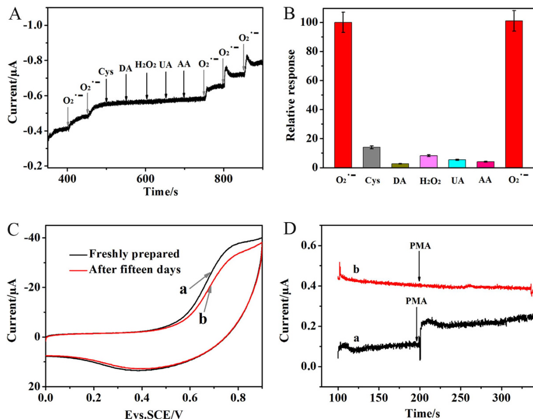
Figure 7. (A) Interference test of SiO 2 -Mn 3 (PO 4 ) 2 /MWCNTs/GCE, (B) The relative response in PBS (pH = 7.4) at 1.0 μM O 2 ·- , 5.0 μM Cys, 5.0 μM DA, 10 μM H 2 O 2 , 10 μM UA and 10 μM AA, (C) CVs of SiO 2 -Mn 3 (PO 4 ) 2 /MWCNTs/GCE, (a) Freshly prepared, and (b) after fifteen days in 0.1 M PBS, Scan rate was 100 mV·s -1 , and (D) Amperometric response of the SiO 2 -Mn 3 (PO 4 ) 2 /MWCNTs/GCE in the (a) presence, and (b) absence of HeLa cells upon sequential additions of PMA to 0.1 M PBS at 0.484 V.
