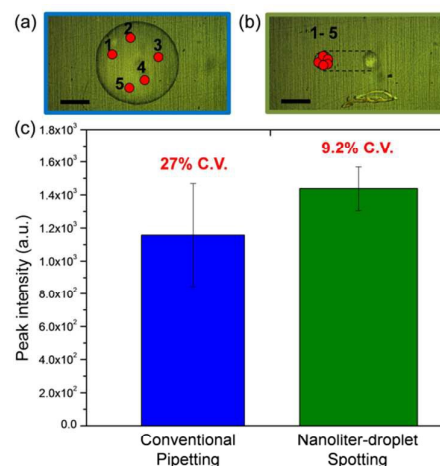
Fig. 3 Photos of dried MALDI spots deposited by (a) pipetting (diameter: 1.5 mm) and (b) PZT spotting (diameter: 300 μm). Approximately 25 times smaller spot (area) was produced when using the PZT nanoliter-droplet ejector (Scale bar = 500 μm). (c) Averages of peak intensities from 5 measurements at different irradiation regions within a spot were compared between two sample deposition manners, coefficient of variations (C.V.= standard deviation/ mean value) were indicated above the error
