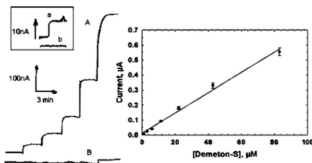
Fig. 2 Current-time traces of screen-printed electrodes modified with OPH mutant (B) and with acid-purified CNT/OPH mutant (A) to 5, 10, 20, 40, and 80 μM demeton-S. Inset shows the response of the sensor at 1 μM demeton-S with (a) and without (b) CNT. Also shown is the calibration curve for demeton-S. Measurement conditions: applied potential 0.4 V vs. Ag/AgCl, pH 7.4 phosphate buffer containing 0.1 M KCl. Each point represents an average of three measurements, and the error bars represent \pm 1 SD. 60
