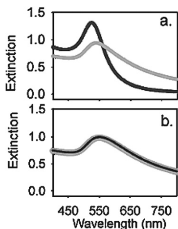
Fig. 3 UV-vis extinction spectra of an active 17E DNAzyme-nanoparticle sensor (a) and an inactive 17Ec DNAzyme-nanoparticle sensor (b) in the absence (light grey curve) or in the presence (dark grey curve) of 5 \mu\text{M} \text{Pb(II)} . 107
