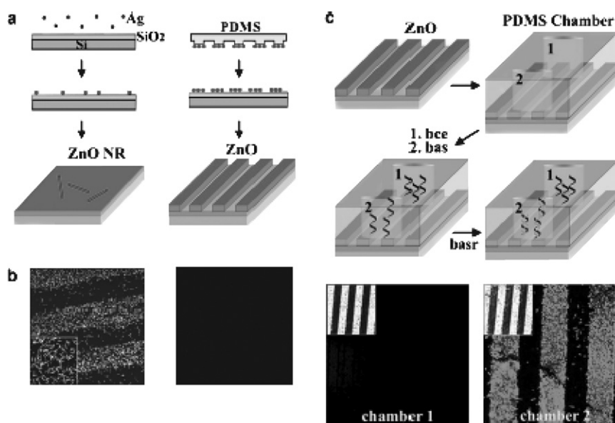
Fig. 6 (a) Schematic illustrations showing simultaneous synthesis and assembly of ZnO nanoplateforms consisting of (left) individual ZnO nanorods and (right) periodically patterned ZnO nanostructures. (b) (Left) SEM image of a patterned ZnO platform with the stripe width and repeat spacing of 50 µm. The inserted SEM image at the bottom left corner shows the lying-down arrangement of ZnO nanostructures inside the patterned stripes. (Right) Confocal fluorescence image taken from the as-synthesized, striped, ZnO nanoplateform where no fluorescence emission was detected. (c) Detection scheme to identify B. anthracis from B. cereus using ZnO nanoplateforms: PDMS chambers were used in order to carry out simultaneous hybridization reactions on the same ZnO nanoplateform. The ZnO nanoplateform contained regularly patterned ZnO stripes with a repeat spacing of 20 µm. Oligonucleotide probes of 5'-GTTACGGAAA GAACCA-3' ( bce ) and 5'-AGTGC GCGAGGAGCCT-3' ( bas ), were first introduced to the reaction chambers 1 and 2, respectively. Subsequently, fluorescein modified basr strands were added to both chambers and allowed to form DNA duplex under the same hybridization conditions. Confocal images taken from these samples showed clear fluorescence emission from chamber 2, in contrast to no discernable fluorescence signal from chamber 1. The insets in the upper left corners of the confocal images are the corresponding bright field images taken from each chamber after the duplex formation reaction. Distinctive fluorescence emission monitored from chamber 2 is due to DNA duplex formation between fully complementary strands of bas and 5'-TCACGCGCTCCTCGGA-3' ( basr ), whereas the lack of duplex formation between mismatching sequences of bce and basr led to no observable fluorescence in chamber 1. The striped patterns of fluorescence emission observed from chamber 2 faithfully mimic the underlying geometry of the ZnO nanoplateform. 127
