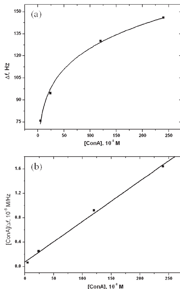
Fig. 2 Frequency change vs. concentration of Con A in 50 mM phosphate buffer at pH 7.0 with 1 mM \text{Ca}^{2+} and 1 mM \text{Mn}^{2+} (a) and its reciprocal plot of [\text{Con A}]/\Delta f vs. [\text{Con A}] (b).
