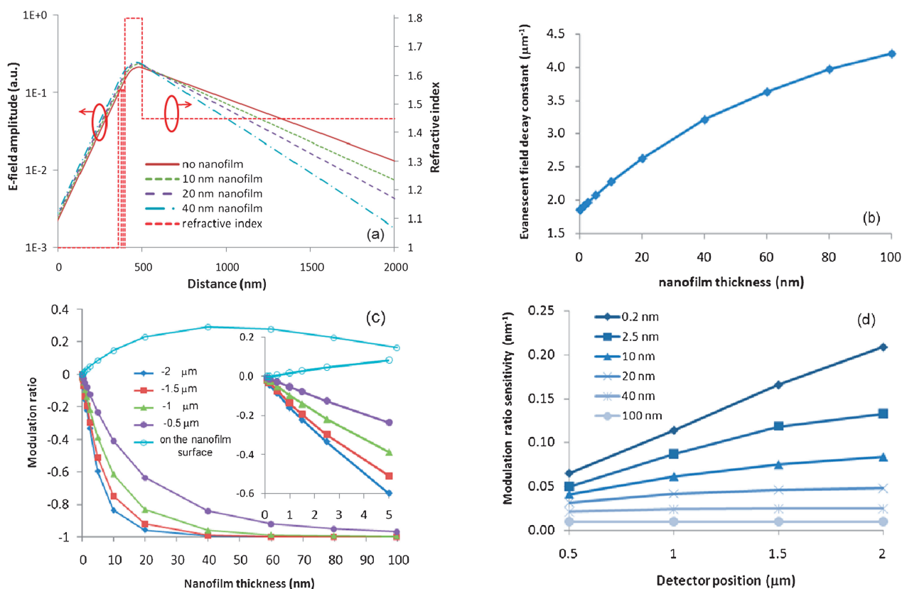
Fig. 2 (a) E-field decays exponentially as a function of depth into the lower waveguide cladding at different rates depending on nanofilm thickness (0–40 nm). The refractive index profile of the waveguide structure is shown (dotted lines) with air as the upper cladding, \text{SiN}_x as the waveguide core, and \text{SiO}_2 as the lower cladding. (b) Evanescent field decay constant dependence on nanofilm thickness. (c) Simulated modulation ratio as a function of nanofilm thicknesses on the waveguide's top surface and for different vertical positions below the waveguide. (d) Sensitivity analysis of the LEAC sensor based on simulation data for different detector positions and film thicknesses.
