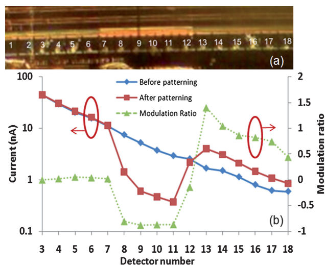
Fig. 4 (a) Photograph of a LEAC sensor waveguide with photoresist patterned above the 7th–12th detectors. (b) Photocurrents measured before (diamonds) and after (squares) the photoresist is patterned as well as the resulting modulation ratio (triangles).
