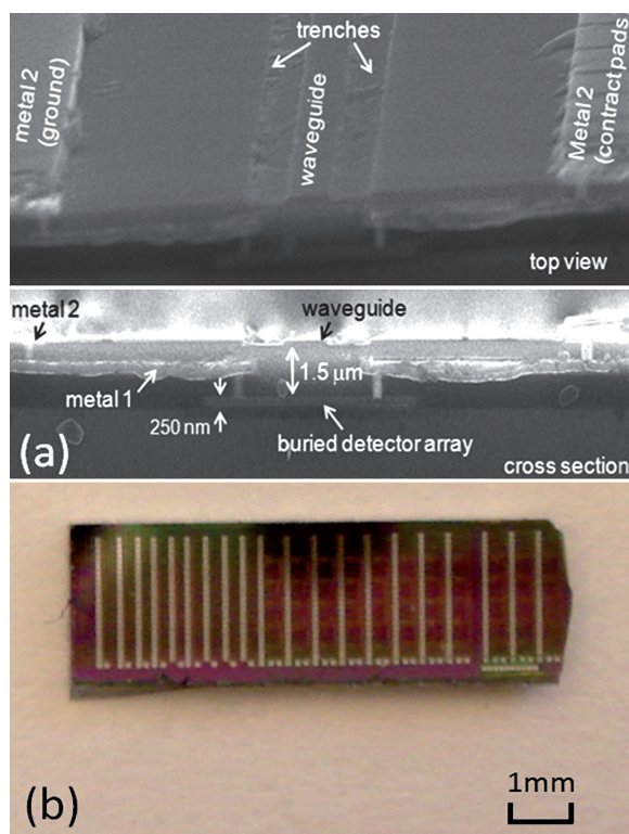
Fig. 3 (a) SEM images of the LEAC biosensor structure incorporating buried detectors. (b) 2.5 mm × 8 mm chip containing 20 biosensor systems consisting of waveguides with integrated detector arrays.
