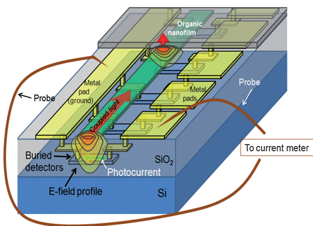
Fig. 1 Schematic diagram of a LEAC biosensor CMOS chip where evanescent field distribution shifts up upon reaching the organic nanofilm, resulting in decreased photocurrent in detectors under the film.
