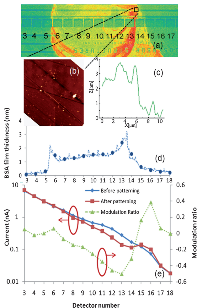
Fig. 5 (a) Fluorescence microscope image of a LEAC sensor waveguide with BSA patterned above the 6th–14th detectors. (b) False intensity AFM topographic image at the indicated position containing the edge of the BSA pattern. (c) Average nanofilm height obtained from AFM data. (d) BSA film thickness along the waveguide (dotted line) and average BSA film thickness above each photodetector (solid circle). (e) Photocurrents measured before (diamonds) and after (squares) the BSA is patterned as well as the photocurrent ratio (triangles).
