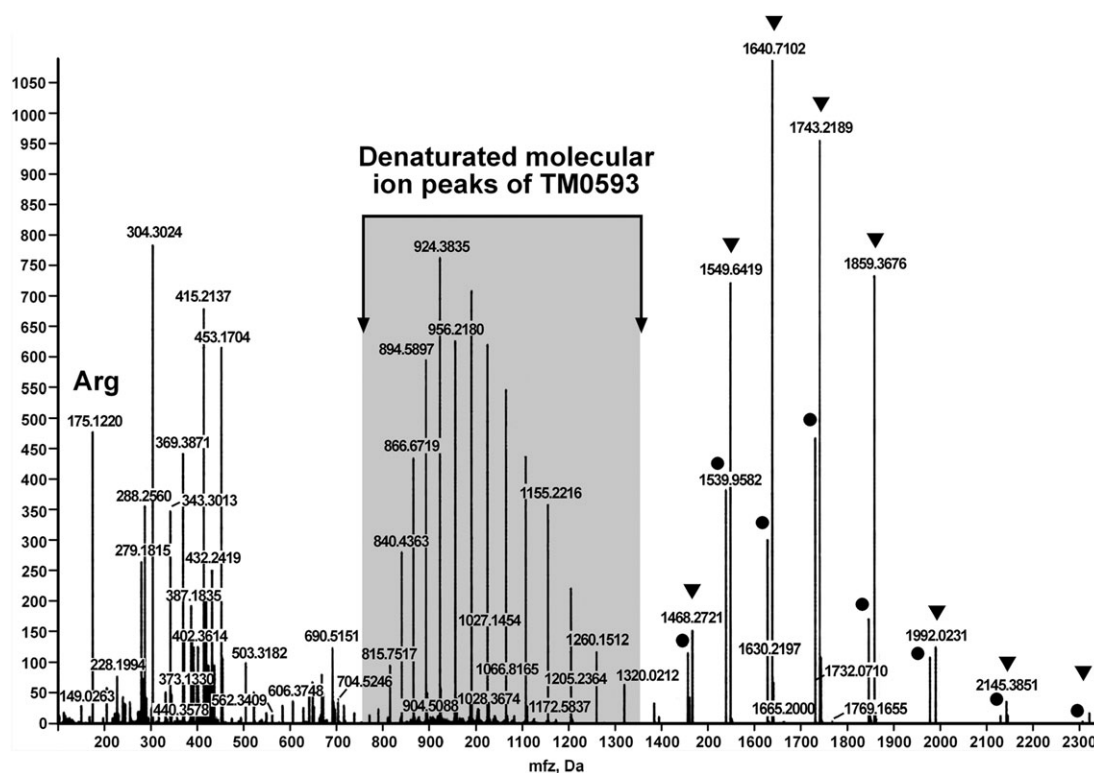
Fig. 3 Nano-ESI mass spectrum of purified TM0593 (10 \mu M) incubated with 20 \mu M arginine in 10 mM ammonium formate. The three distinct charge distributions in the spectrum correspond to native TM0593 (circles), denatured TM0593 (shaded), and native TM0593 plus Arg (triangles).
