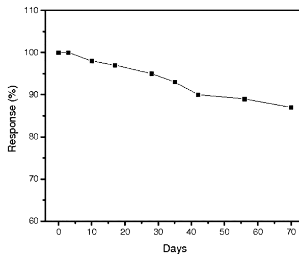
Fig. 7 Study on stability of the Au-BMI·PF 6 biosensor using 4.798 \mu M luteolin in 0.1 M acetate buffer solution (pH 4.0).
