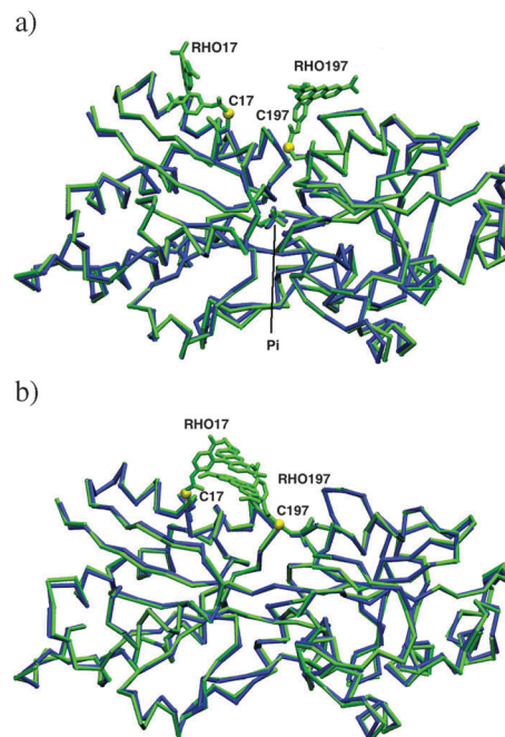
Fig. 2 (a) RHO 2 -PBP-Pi: superposition of C α trace representations of the initial structure (blue), derived from X-ray experiments 2,27,28 and final MD structure (green). The protein is a single chain with two domains consisting of \alpha -helix and \beta -sheet elements. 2,27 The deep cleft in between tightly binds the analyte Pi. The two RHO fluorophores (residue names RHO197 and RHO17) are largely separated from each other. (b) RHO 2 -PBP: superposition of initial (blue) and final (green) structures of classical MD simulations for RHO 2 -PBP. The two RHO fluorophores RHO197 and RHO17 maintain a stable stacked 'face A to face B' dimer configuration. Face A is that side of the xanthylium system adjacent to the carboxylate group on the pendant aryl ring, whereas face B is the side of the xanthylium system that is distal to the carboxylate.
