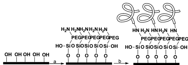
Scheme 1 Surface functionalization. (a) \text{NH}_2\text{-PEG-Si(OEt)}_3 , EtOH : \text{H}_2\text{O} 95 : 5, 2 h at rt, (b) proteins 2 M, desalted buffer, EDC, 12 h, 4 °C.
