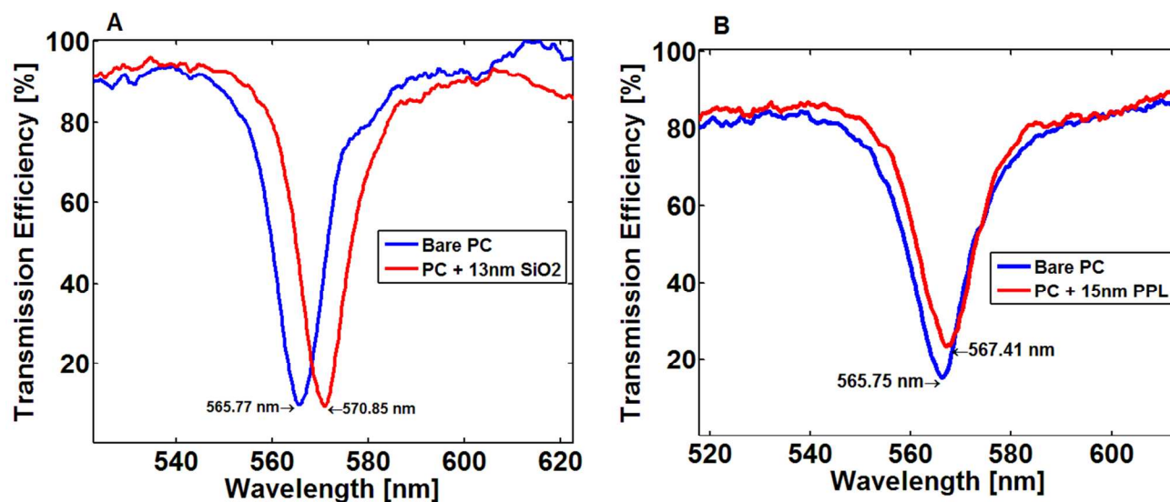
Figure 5. A. Normalized transmission characteristics for a bare PC and an adjacent region of the same PC coated with a SiO 2 thin film, resulting in a positive shift of the measured PWV. B. Transmission spectra of a PC before and after deposition of a monolayer of PPL protein.
