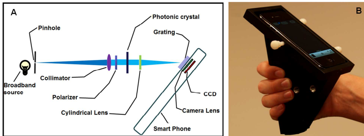
Figure 2. A. Schematic of the optical components within the smartphone cradle. Broadband light from an external source (such as an incandescent lamp or LED) is collimated by the combination of an entrance pinhole and a collimating lens. After passing through a linear polarizing filter, light passes through the PC, which resonantly reflects one narrow band of wavelengths. The cylindrical lens increases the amount of light that is collected by the camera. B. Photo of the cradle with a PC biosensor slide inserted into the detection slot.
