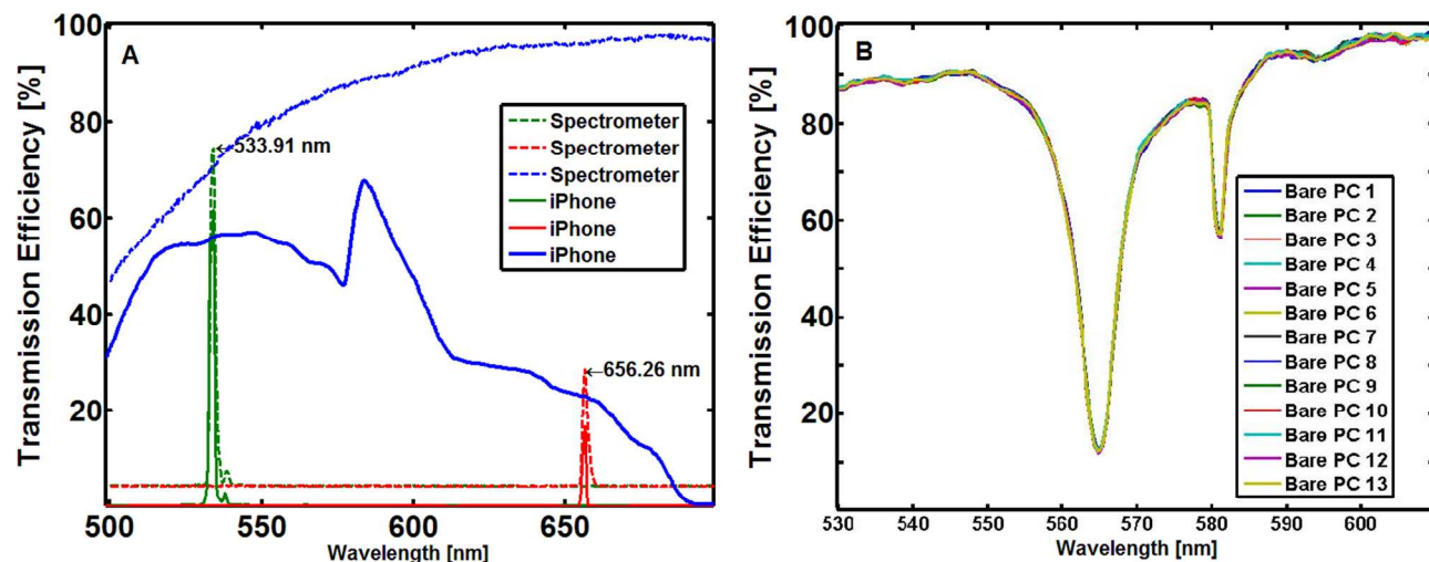
Figure 4. A. Overlaid spectra from red and green laser pointers measured with a calibrated spectrometer (dashed curves) and the smartphone (solid curves) used to obtain a translation factor from pixels to wavelength values. B. The transmission spectra of 13 independent PC spectra taken by removing and re-inserting the PC into the cradle, demonstrating excellent measurement reproducibility.
