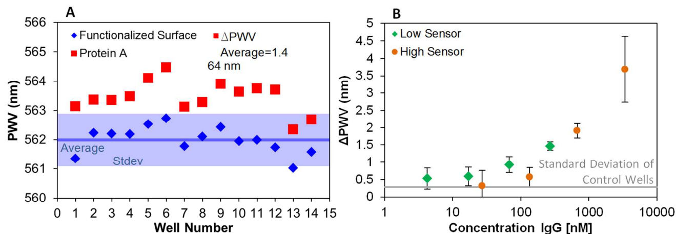
Figure 6. Concentration Dependent PWV Shift of Porcine IgG Antibody. A. Variation in slide functionalization versus Protein A deposition. B. Protein A was immobilized on two PC sensors to detect concentrations of porcine IgG antibody present in quantities between 1 nM and 5000 nM. N=3 for assay wells; N=2 for control wells.
