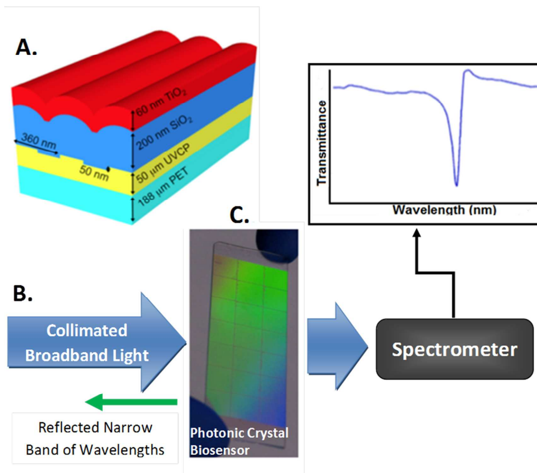
Figure 1. A. Cross section schematic of the PC structure. B. Operating principle of the PC biosensor. When the structure is illuminated with a wide range of wavelengths, only a narrow band of wavelengths is reflected, while all other wavelengths transmit through without attenuation. C. Photograph of a photonic crystal attached to a 1x3 in 2 glass microscope slide.
