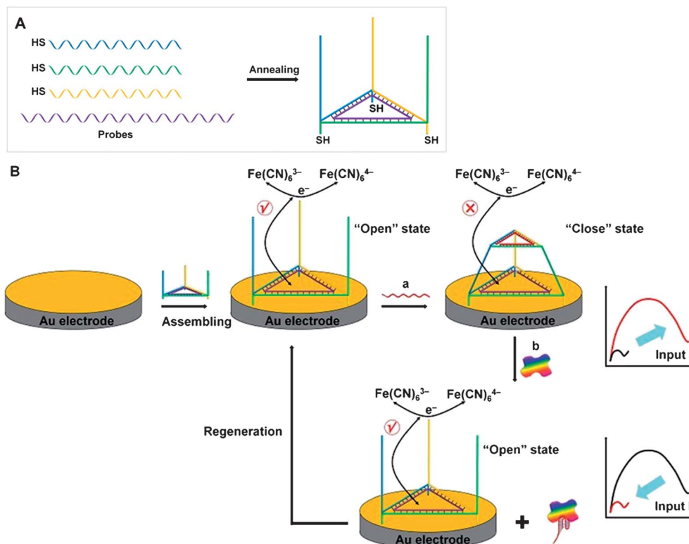
Fig. 1 (A) Schematic illustration of the ET DNA (Equilateral Triangle DNA) nanostructure. The ET DNA was self-assembled in equal stoichiometric amounts of three thiolated 36-nt DNA fragments and one 55-nt DNA fragment. (B) Schematic representation of the biosensing process based on the “Closed” and “Open” states during the conversion between the ET DNA and TPF DNA nanostructures assembled on an Au electrode (a: aptamer, b: target).
