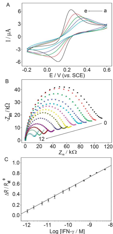
Fig. 5 (A) CVs of the "Closed" state of TPF_{DNA} modified Au electrodes in a 1.0 mM Fe(CN)_6^{3-/4-} (containing 0.1 M NaCl) solution corresponding to (a) 0, (b) 5.0 \times 10^{-12} , (c) 5.0 \times 10^{-11} , (d) 5.0 \times 10^{-10} , and 5.0 \times 10^{-9} M IFN- \gamma . (B) FIS curves of the TPF_{DNA} modified Au electrodes in a 1.0 mM Fe(CN)_6^{3-/4-} (containing 0.1 M NaCl) solution corresponding to different concentrations of IFN- \gamma (from 0 to 12: 1.0 \times 10^{-12} , 2.0 \times 10^{-12} , 5.0 \times 10^{-12} , 1.0 \times 10^{-11} , 2.0 \times 10^{-11} , 5.0 \times 10^{-11} , 1.0 \times 10^{-10} , 2.0 \times 10^{-10} , 5.0 \times 10^{-10} , 1.0 \times 10^{-9} , 2.0 \times 10^{-9} , and 5.0 \times 10^{-9} M). (C) The corresponding calibration plot of \Delta R/R_{et}^0 vs. IFN- \gamma concentrations.
