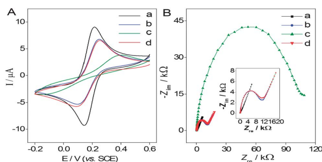
Fig. 3 CVs (A) and FIS (B) of the (a) bare and (b–d) DNA nanostructure modified electrodes in a 1.0 mM Fe(CN) 6 3−/4− (containing 0.1 M NaCl) solution. (b) The initial "Open" state of ET DNA , (c) the middle "Closed" state of TPF DNA , and (d) the reset to the "Open" state of ET DNA . Scan rate: 50 mV s −1 . Applied potential: +0.179 V (vs. SCE). Frequency range: 10 mHz to 10 kHz. Amplitude: 5 mV.
