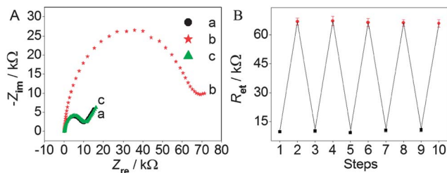
Fig. 4 (A) FIS curves of the reversible changes of the electron-transfer resistance upon "Open"/"Closed" functions. (a) The initial "Open" state of ET_{DNA} , (b) the middle "Closed" state of TPF_{DNA} , and (c) the reset to the "Open" state of ET_{DNA} . The experiment was performed upon application of the biasing potential of +0.179 V (vs. SCE). (B) Reversible changes of the R_{et} values upon "Open"/"Closed" functions.
