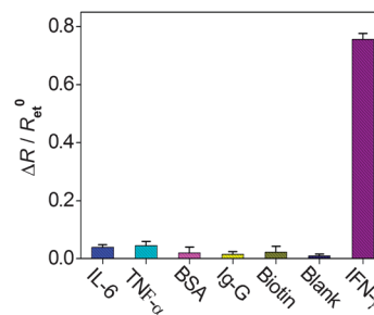
Fig. 6 Specificity of the biosensor for IFN- \gamma detection over the same concentration of 1.0 nM IL-6, TNF- \alpha , BSA, IgG, and biotin. The error bars represent the standard deviations of triplicate measurements.
