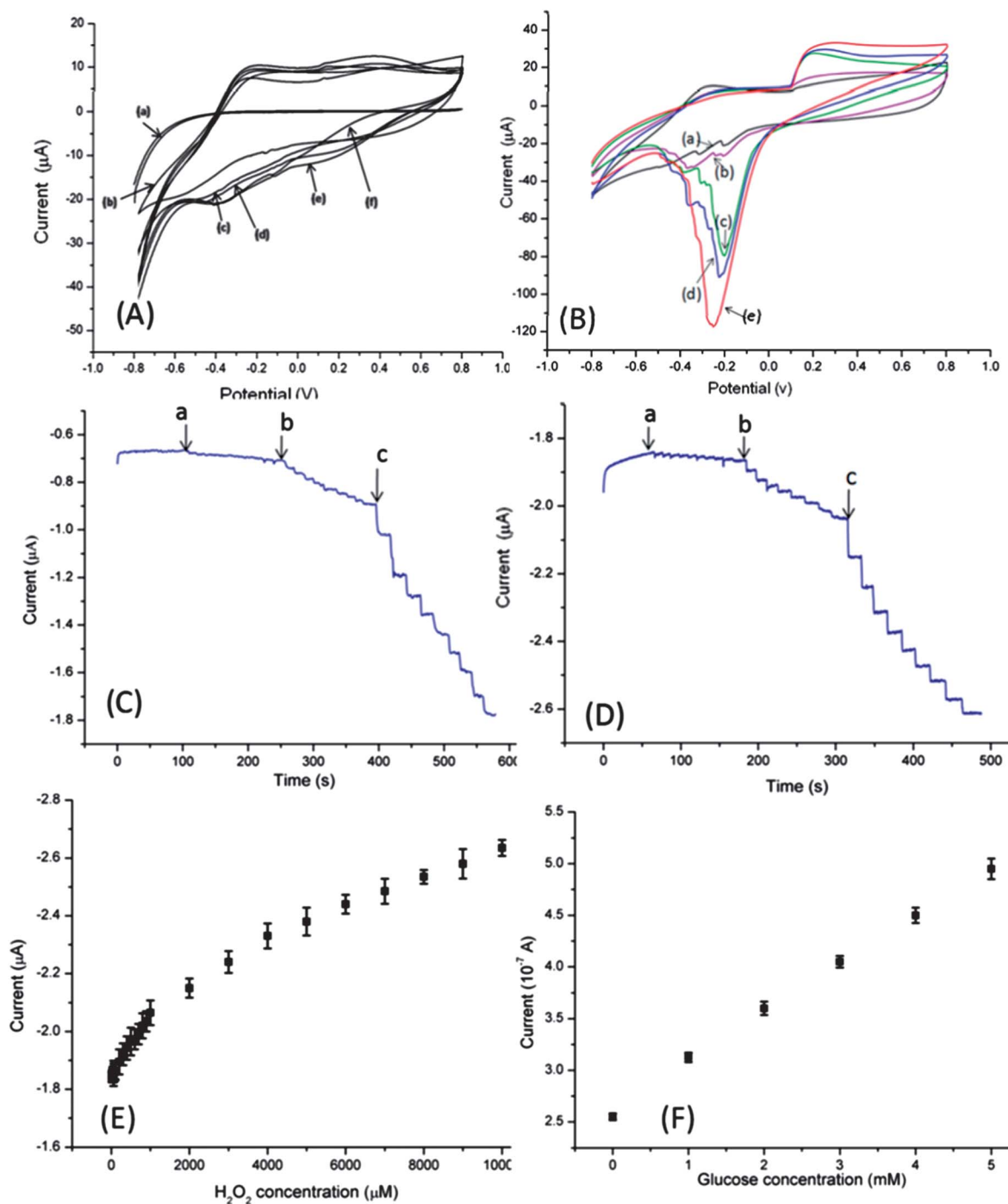
Fig. 4 (A) CVs of bare and modified SPCEs in 0.01 M PBS with \text{H}_2\text{O}_2 concentrations as stated. The potentials are vs. Ag/AgCl (3.0 M NaCl). Scan rate: 0.1\text{ V s}^{-1} (a) Bare SPCE; (b to f) Single layer PPy film in 0, 1, 10, 100 and 1000\text{ }\mu\text{M} \text{H}_2\text{O}_2 , respectively; (B) CVs of single layer inkjet printed PPy/HRP film in 0.01 M PBS, (a–e) 0, 1, 10, 100 and 1000\text{ }\mu\text{M} \text{H}_2\text{O}_2 , respectively. HRP loading is 2.5\text{ mg mL}^{-1} . The potentials are vs. Ag/AgCl (3.0 M NaCl). Scan rate: 0.1\text{ V s}^{-1} ; chronoamperograms of (C) single layer inkjet printed PPy/HRP film and (D) five layers inkjet printed PPy/HRP film. Applied potential: -0.2\text{ V} . HRP loading: 2.5\text{ mg mL}^{-1} . a–c are the starting points of the addition of 10^{-5} , 10^{-4} and 10^{-3}\text{ M} \text{H}_2\text{O}_2 ; (E) The calibration curve of the five layers PPy/HRP biosensor to \text{H}_2\text{O}_2 from 10^{-5} to 10^{-2}\text{ M} and (F) the calibration curve of a single layer PPy/GoD biosensor to glucose from 1 to 5 mM. Error bars represent RSD of five measurements.
