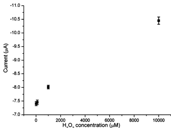
Fig. 5 The reproducibility calibration curve of five single layer inkjet printed PPy/HRP biosensors. Error bars represent RSD of single measurement of five sensors.
