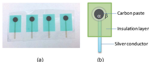
Fig. 1 (a) Strip of four bare SPCEs on Polyethylene terephthalate (PET) and (b) Schematic of the inkjet printed PPy/enzyme biosensor based on an SPCE. (α) inner black circle: PPy/enzyme film on carbon paste (diameter: 5.5 mm); (β) outer white circle covering inner black circle: EC membrane covering PPy/enzyme electrode (diameter: 7 mm).
