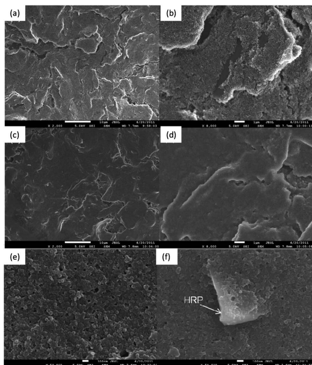
Fig. 2 (a) SEM image of bare SPCE, scale bar: 10 \mu\text{m} ; (b) SEM image of bare SPCE, scale bar 1 \mu\text{m} ; (c) SEM image of one layer of PPy film on SPCE, scale bar, 10 \mu\text{m} ; (d) SEM image of one layer of PPy film on SPCE, scale bar, 1 \mu\text{m} ; (e) PPy nanoparticles that constituted 1 layer PPy/HRP film, scale bar: 100 \text{ nm} and (f) detail of PPy particles encapsulating HRP enzyme crystal, scale bar 100 \text{ nm} .
