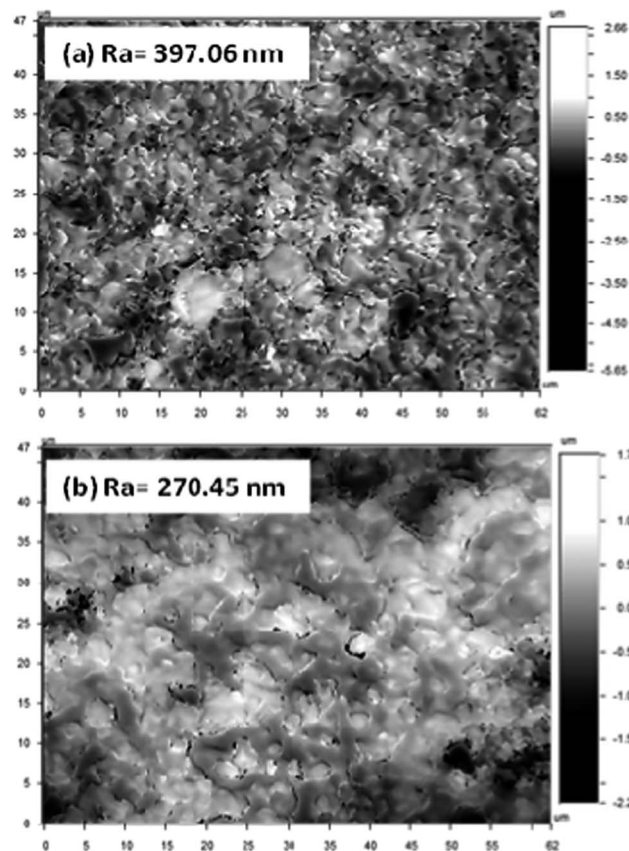
Fig. 3 Profilometry images and average roughness of (a) Bare SPCE and (b) single layer PPy film on SPCE.
