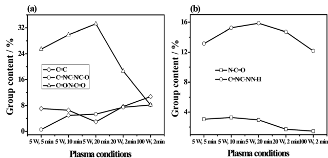
Fig. 4 Relative intensity of functional (a) carbon-related and (b) nitrogen-related groups of G-PPAA deposited at 5 W (5, 10, and 20 min), 20 W (2 min), and 100 W (2 min).
