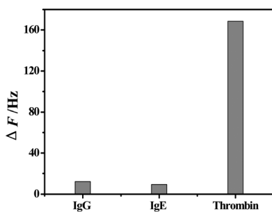
Fig. 11 \Delta F of the detection of 10 ng mL -1 thrombin, 100 ng mL -1 IgG and 100 ng mL -1 IgE.
