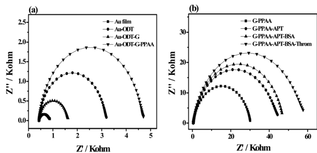
Fig. 7 Nyquist diagrams of EIS for (a) each stage of G-PPAA films deposited at 5 W on a Au wafer self-assembled with ODT and (b) the immobilization of aptamer and the detection of thrombin on the surface of G-PPAA film.
