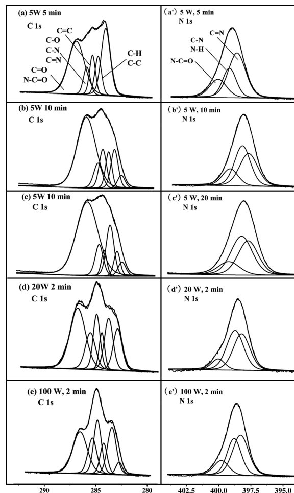
Fig. 3 C1s and N1s core-level XPS spectra and their corresponding peaks in the G-PPAA films deposited at 5 W (5, 10, and 20 min), 20 W (2 min), and 100 W (2 min).
