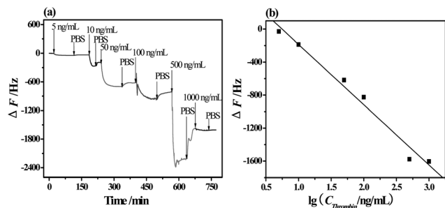
Fig. 10 (a) Frequency response profiles for the detection of thrombin at different concentrations of 5, 10, 50, 100, 500 and 1000 ng mL -1 . (b) Linear calibration curve for \Delta F versus \lg(C_{\text{thrombin}} / \text{ng mL}^{-1}) , where C_{\text{thrombin}} is the concentration of thrombin.
