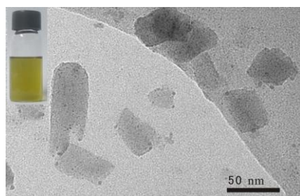
Fig. 1. Typical TEM image of prepared \text{MoS}_2 nanosheets and photograph of a typical chemically exfoliated \text{MoS}_2 suspension in water.
