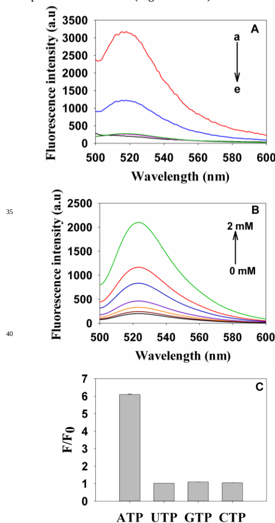
Fig. 3. (A) Fluorescence emission spectra of P1 and P3 under different conditions: (a) P1; (b) P1 + \text{MoS}_2 + ATP; (c) P3 + \text{MoS}_2 + ATP; (d) P3 + \text{MoS}_2 ; (e) P1 + \text{MoS}_2 ( \text{MoS}_2 40 \mu\text{g mL}^{-1} , P1 50 nM, P3 50 nM, ATP 1 mM). (B) Fluorescence emission spectral responses of DNA- \text{MoS}_2 nanosheet biosensor to varying concentrations of ATP, 0, 10, 50, 100, 500, 1000, and 2000 \mu\text{M} , respectively. (C) Peak fluorescence intensity enhancement ( F/F_0 ) of DNA- \text{MoS}_2 nanosheet biosensor in the presence of 1000 \mu\text{M} ATP, UTP, GTP or CTP, respectively ( \text{MoS}_2 40 \mu\text{g mL}^{-1} , P1 50 nM).
