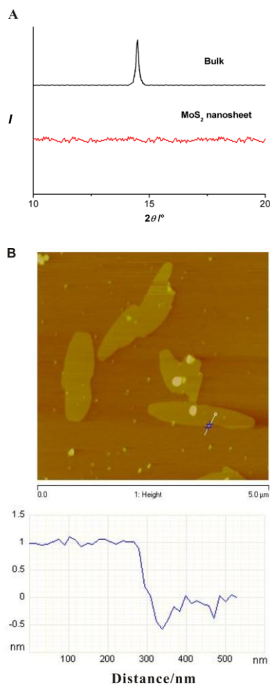
Fig. 2. (A) Comparison of XRD patterns of bulk \text{MoS}_2 and \text{MoS}_2 nanosheets. (B) Typical AFM image and associated height profile of \text{MoS}_2 nanosheets.
