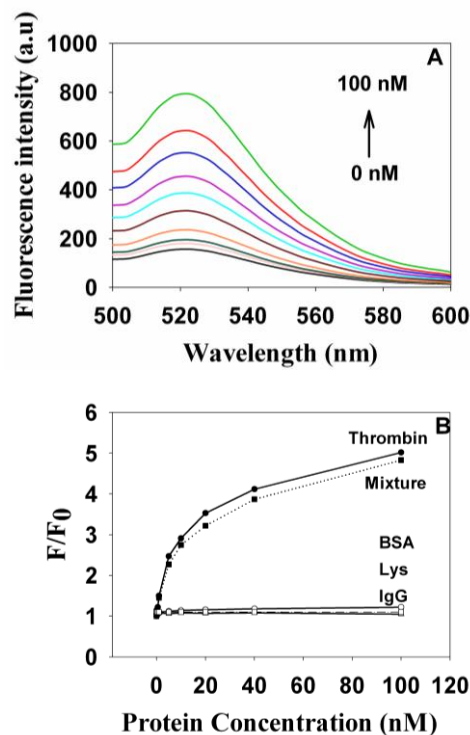
Fig. 4. (A) Fluorescence emission spectra of DNA–MoS 2 nanosheet biosensor in the presence of increasing amounts of thrombin. The arrow indicates the signal changes with increases in thrombin concentrations (0, 0.5, 1, 2, 3, 5, 10, 65 20, 40, 100 nM). (B) Fluorescence enhancements ( F/F_0 ) of DNA–MoS 2 nanosheet biosensor in the Tris–HCl buffer by increasing concentrations of thrombin (●), BSA (○), Lys (□), and IgG (△), separately, as well as a mixture of proteins (concentrations of proteins were 100 nM) with increasing concentrations of thrombin (■). Fluorescence intensity ratio F/F_0 plotted 70 against the concentration of protein, where F and F_0 are the fluorescence intensity with and without protein (MoS 2 40 \mu\text{g mL}^{-1} , P2 20 nM).
