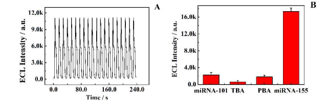
Fig. 6. (A) The stability of the prepared ECL biosensor incubated with 0.5 pM miRNA under consecutive cyclic potential scans for 20 cycles in 2 mL PBS (pH 7.4) with 1.00\times10^{-4} M luminol and 0.7\ \mu\text{M} H_2O_2 . (B) Comparison of ECL responses with 500 pM of miRNA-101, 500 pM of TBA, 500 pM of PBA, 50 pM of miRNA-155.
