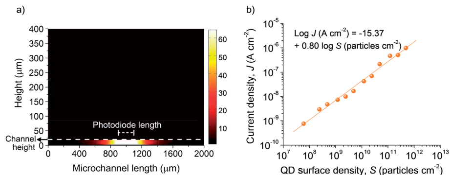
Fig. 2 (a) Scheme derived from the optical model demonstrating the zones of photons emitted by the QDs, within the microchannel, that diffuse into the detector. (b) Photoresponse of the a-Si:H photosensor plotted as a function of the surface density of QDs.
