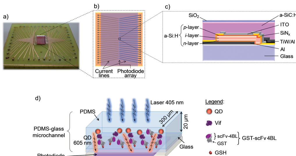
Fig. 1 (a and b) The 23-photodiode sensor chip mounted on a printed circuit board. (c) Cross sectional schematic view of the a-Si:H PIN photodetector. (d) Schematic of the biorecognition reactions of the probe (GST-scFv 4BL) with the target protein (Vif) labeled with quantum dots (QDs) within the microchannel. a-Si:H, amorphous silicon-carbon filter; ITO, indium tin oxide top contact, Al, aluminum bottom contact; SiNx, silicon nitride insulator film; SiO 2 , silicon dioxide insulator film.
