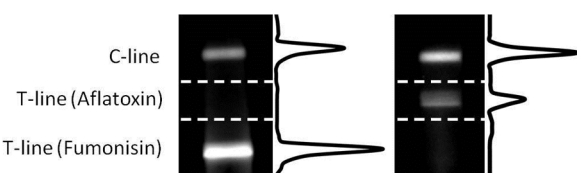
Fig. 2 Chemiluminescence images and intensity profile of nitrocellulose membranes in which anti-Aflatoxin and anti-Fumonisin antibodies separately ran in the absence of analytes.
