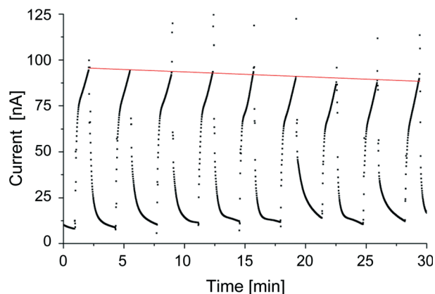
Fig. 4 Current profile of the AChE biosensor during alternating dipping into the enzyme substrate acetylthiocholine (ATCh) and buffer using the AutoDip cartridge (sensor 2). The decline of the peak heights over time is visualized by the red line. Outliers appearing above the line were generated during switching and are not considered when determining peak heights.
