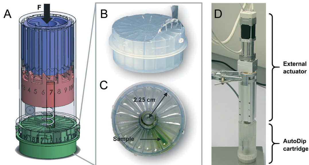
Fig. 2 Detailed AutoDip design and evaluation model. (A) 3D drawing of the AutoDip cartridge. (B) Image of the reagent module fabricated by stereolithography and sealed with peelable foil. (C) Top view of the reagent module pre-filled with reagents and a homogenized food sample (green). (D) Prototype of the AutoDip cartridge with an external vertical actuator.
