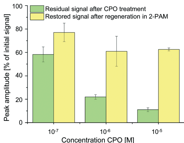
Fig. 6 Pesticide detection in buffer. Residual signals after incubation of the biosensor in buffer with pesticide CPO in three different concentrations (green). Restored signal after regeneration of the biosensor in 2-PAM (yellow). Each column represents a mean value of three independent experiments. Error bars indicate standard deviations.
