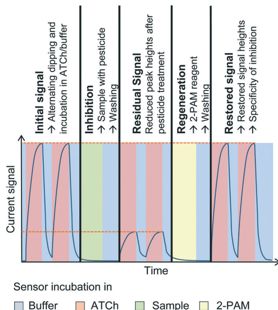
Fig. 3 Schematic of the current profile of the electrochemical pesticide detection assay with an acetylcholinesterase biosensor. ATCh (red): acetylthiocholine, the substrate for the enzyme reaction; buffer (blue) for equilibrating and washing the sensor; sample with pesticide (green); 2-PAM (yellow): pralidoxime, the regeneration reagent. Current peaks are generated by incubation of the sensor in ATCh for a defined time and subsequent dipping of the sensor into buffer. A repetition of this sequence demonstrates reproducibility of the signal.
