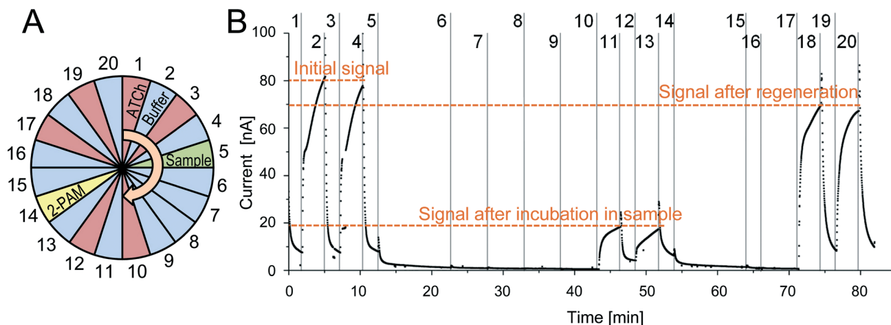
Fig. 5 Reagent scheme and corresponding current profile of a complete pesticide assay in the AutoDip cartridge. (A) Loading scheme of the prefilled reagent module. The arrow indicates the starting point and the rotational direction of the sensor. ATCh (red), buffer (blue), sample (green), 2-PAM (yellow). The numbers show the process steps for the ball-pen mechanism. (B) Complete pesticide assay with 10^{-6} M CPO in buffer as a sample. The numbers refer to the reagent cavities in (A). Reduction of the signal after incubation in the sample and regeneration after incubation in 2-PAM indicate the presence of CPO.
