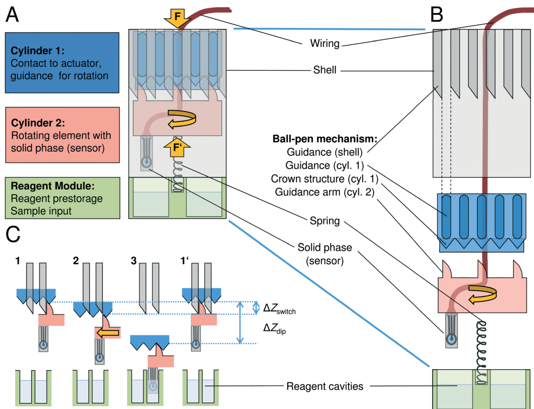
Fig. 1 Schematic drawing (A, B) and functional principle (C) of the AutoDip cartridge. (A) A static shell encloses two vertically movable cylinders. The rotation of cylinder 2, positioning the solid phase, is controlled by pen mechanics. Vertical movement and thereby operation of the ball-pen mechanism is directed by the interplay of a mechanical force ( F ) applied to cylinder 1 by an external actuator and a counter acting spring force ( F' ). (B) Explosion view of the cartridge. (C) Rolled up view of the cartridge to illustrate the principle of rotational transport of the solid phase from one reagent cavity to another. The displacement that must be provided by the actuator for switching and dipping is illustrated by \Delta Z_{\text{switch}} and \Delta Z_{\text{dip}} , respectively. See text for the detailed description.
