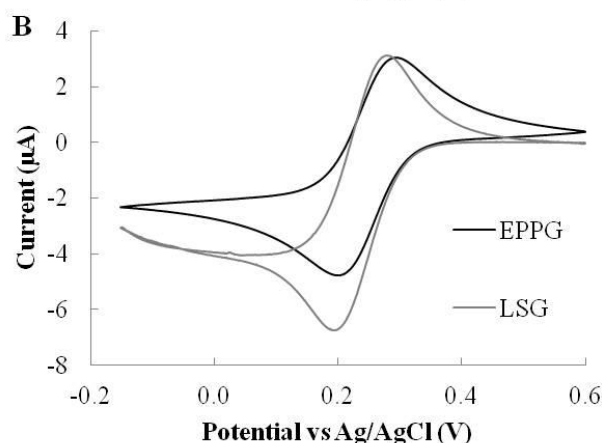
Fig. 5. Panel A shows cyclic voltammograms of 1,1'-ferrocene dimethanol and panel B potassium ferricyanide at a scan rate of 10 \text{ mV s}^{-1} at EPPG electrode surfaces compared to the disposable planar three electrode LSG system.
