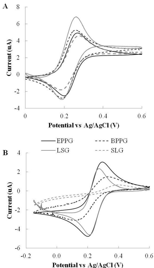
Fig.2. Cyclic voltammograms of (A) 1,1'-ferrocene dimethanol and (B) potassium ferricyanide in 1M KCl at a scan rate of 10 mV s -1 at unmodified 3 mm diameter EPPG, BPPG, LSG and SLG electrode surfaces.
