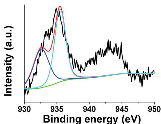
Fig. 5 Cu 2p XPS spectrum of synthesized C-rich ssDNA-Ag NCs in the presence of \text{Cu}^{2+} ions solution (1 mM).
