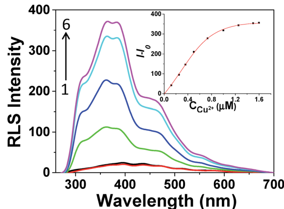
Fig. 2 Resonance light scattering (RLS) spectra of C-rich ssDNA templated silver nanoclusters in the absence and presence of the various concentrations of copper(II) ions solution at room temperature. Conditions: (1) (black line), the buffer solution; (2) (red line), C-rich ssDNA-Ag NCs; (3–6): 2 + Cu 2+ ions ( \mu\text{M} ): 0.125 (green line), 0.375 (blue line), 0.75 (cyan line), 1.5 (magenta line). The inserted figure reveals the plot of the increment of the resonance light scattering intensity of C-rich ssDNA-Ag NCs versus the concentration of copper(II) ions.
