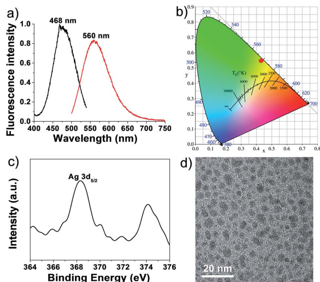
Fig. 1 (a) The excitation (black) and emission (red) spectra of ssDNA templated silver nanoclusters. The template is C-rich ssDNA (5'-(CCCTAA) 3 CCCTA-3'). The DNA sequence is shown in 5'-3'. (b) The image of CIE1931 chromaticity coordinate calculation of C-rich ssDNA templated Ag NCs (C-rich ssDNA-Ag NCs). (c) Ag 3d XPS spectrum of C-rich ssDNA-Ag NCs. (d) TEM image of the synthesized C-rich ssDNA-Ag NCs, scale bar: 20 nm.
