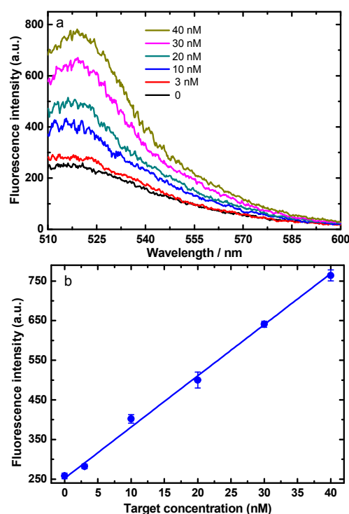
Fig.7 Fluorescence response of samples without HP2 and HCRs (50 nM HP1 and 60 \mu\text{g/mL} MoS 2 ) for different concentrations of the target DNA. (a) Fluorescence emission spectra. (b) Relationship between the fluorescence intensity at the emission wavelength of 520 nm and the target DNA concentration ranging from 0 to 40 nM. All the samples reacted at 24 ^{\circ}\text{C} for 3 h before measurement.
