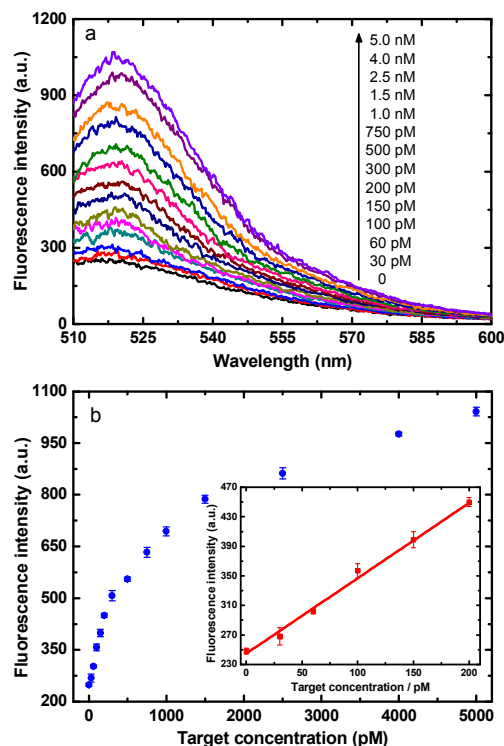
Fig.6 Fluorescence response of the proposed sensing system (50 nM HP1, 50 nM HP2, and 60 \mu\text{g/mL} MoS 2 ) in the presence of different amounts of target DNA. (a) Fluorescence emission spectra. (b) Fluorescence intensity at the emission wavelength of 520 nm as a function of target DNA concentration. The inset shows the linear relationship in the concentration range from 0 to 200 pM. All the samples reacted at 24 ^{\circ}\text{C} for 3 h before measurement.
