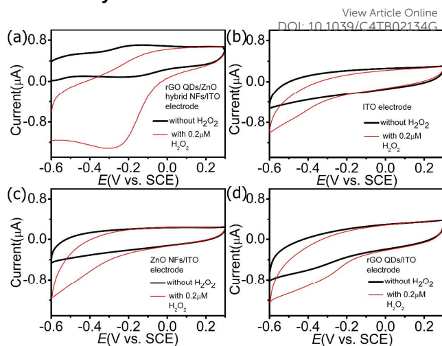
Figure 3. Voltammetric responses of the rGO QDs/ZnO hybrid NFs/ITO (a), ITO (b), ZnO NFs/ITO (c), and rGO QDs/ITO electrodes (d) in N 2 -saturated PBS (0.1 M, pH 7.2) with (red curve) and without (black curve) 0.2 μM H 2 O 2 . Scan rate was 100\text{ mV s}^{-1} .
