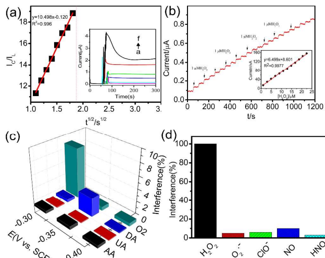
Figure 4. (a) Chronoamperograms obtained at the rGO QDs/ZnO hybrid NFs/ITO in the (a) absence and presence of (b) 5, (c) 70, (d) 120, (e) 250, and (f) 350 nM of H_2O_2 , first and second potential steps were -0.6 and -0.3 V vs. SCE, respectively. Left: dependence of I_c/I_L on t^{1/2} derived from the data of chronoamperograms of (a) and (f) in the main panel. (b) Amperometric i-t response at rGO QDs/ZnO hybrid NFs upon successive additions of 1–22 \mu\text{M} H_2O_2 into continuously stirred N_2 saturated 0.1 M PBS (pH 7.2). Applied potential: -0.4 V. Inset (below) is the plot of response current vs. [H_2O_2] . (c) The typical selectivity profile of the present biosensor obtained at different applied potentials: -0.3, -0.35, -0.4 V versus SCE (derived from the data of Figure S3). (d) ROS selectivity obtained at -0.4 V versus SCE.
