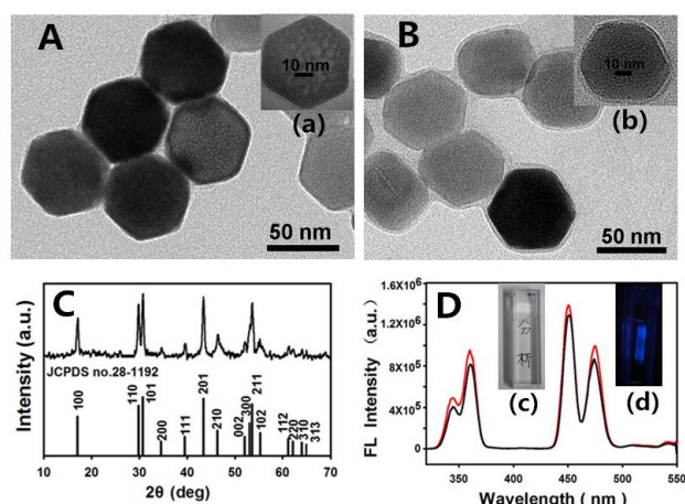
Fig. 1 TEM images of the (A) OA-UCNPs in cyclohexane and (B) DNA-modified UCNPs in water. (The inset shows the high-resolution TEM images of the respective samples). (C) X-ray diffraction pattern of NaYF 4 :Yb,Tm@NaYF 4 nanocrystals. (D) Upconversion fluorescence spectra of the OA-UCNPs (red curve) and DNA-UCNPs (black curve). (The inset shows a photograph of the DNA-UCNPs in water under ambient light (c) and irradiated by 980 nm light (d)).
