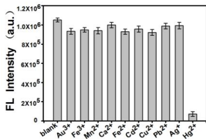
Fig. 4 Selectivity of the analysis of \text{Hg}^{2+} ions by the method depicted in Scheme 1 with the following metal ions: \text{Au}^{3+} ; \text{Fe}^{3+} ; \text{Mn}^{2+} ; \text{Ca}^{2+} ; \text{Fe}^{2+} ; \text{Cd}^{2+} ; \text{Cu}^{2+} ; \text{Pb}^{2+} ; \text{Ag}^{+} ; \text{Hg}^{2+} . The concentration of \text{Hg}^{2+} was 10 \mu\text{M} . The concentrations of the other metal ions were 100 \mu\text{M} . The error bars represented standard deviation of three repetitive experiments.
