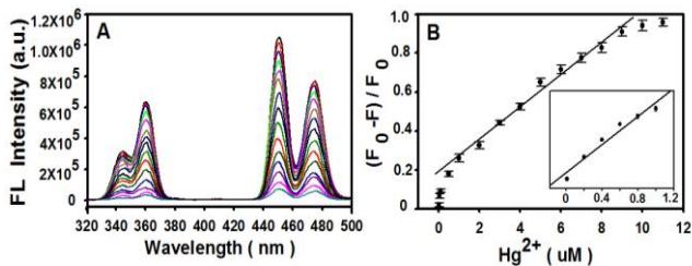
Fig.3 (A) Upconversion fluorescence spectra of the biosensor with varying concentrations of \text{Hg}^{2+} ions. (B) Linear relationship between the fluorescence quenching efficiency and the concentrations of \text{Hg}^{2+} ions within the range of 10 nM-10 \mu\text{M} . The error bars represented the standard deviations of three independent experiments.
