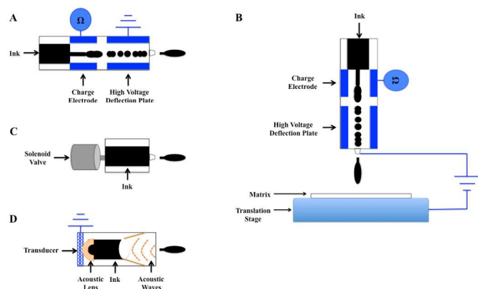
Fig. 6 Other drop-on-demand inkjet printers. A: electrostatic inkjet printer; B: electrohydrodynamic inkjet printer; C: valve inkjet printer; D: acoustic inkjet printer.
