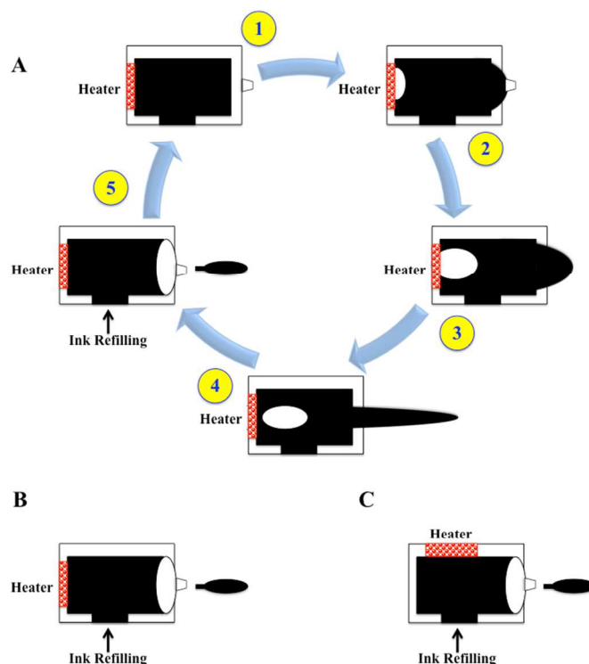
Fig. 4 Drop-on-demand thermal inkjet printer. A: Mechanism. Ink is rapidly heated to a high temperature to vaporize which creates a bubble at the surface of a heater causing a pressure pulse that exudes ink droplets through the nozzle. The vapor bubble collapses, as the ink droplets are ejected, thereby generating a force to refill the ink; B: Thermal “roof-shooter” configuration; C: Thermal “side-shooter” configuration.
