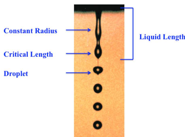
Fig. 1 Lord Rayleigh's idea of instability of jets. From Ref. 9 . Copyright 2001 Society of Photo Optical Instrumentation Engineers.
