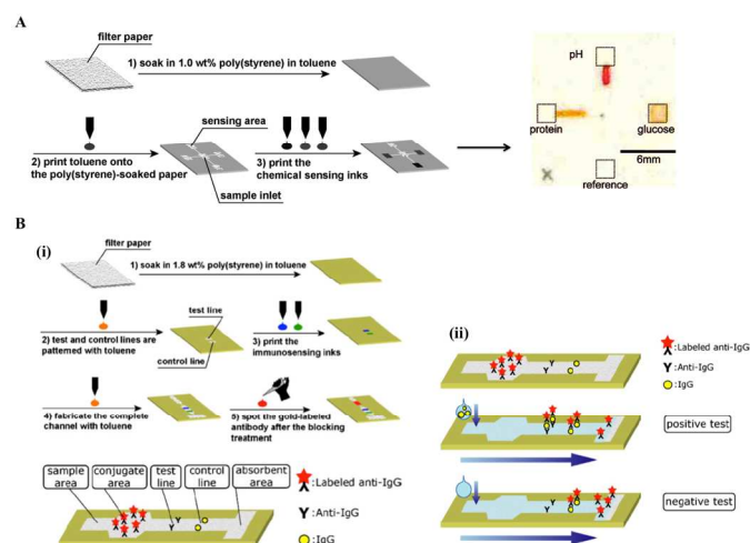
Fig. 11 Inkjet fabricated biosensors with indirect channel or zone patterning. A: schematic representation of the fabrication process of the inkjet printed multi-analyte biosensor. From Ref. 63 . Copyright 2008 American Chemical Society. B: (i) schematic representation of the fabrication process of the inkjet printed unassembled lateral flow biosensor. (ii) Reaction scheme of the sandwich assay. From Ref. 83 . Copyright 2008 Springer-Verlag.
