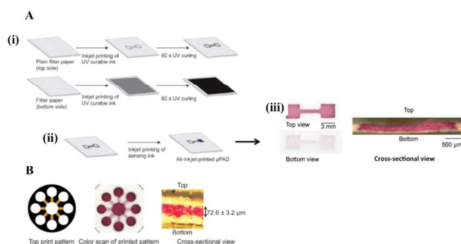
Fig. 13 Inkjet fabricated biosensors with direct channel or zone patterning by hydrophobic fencing. A: schematic representation of the fabrication process of the inkjet printed peroxide biosensor (i) patterning of the filter paper by a double-sided printing process (grey and black colors indicate the printed hydrophobic features before and after UV curing, respectively). (ii) Inkjet printing of peroxide sensing ink. (iii) Color-scanned images of the inkjet printed peroxide biosensor with a bottom cover by top, cross-sectional, and bottom views. B: inkjet printed peroxide biosensor with both a top and a bottom cover. Reproduced from Ref. 84 with permission from the Royal Society of Chemistry.
