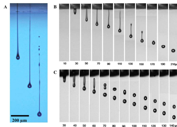
Fig. 8 Satellite droplets of inkjet printing. A: a high-speed photographic image showing three drops ejected from a DOD printer at different stages of drop formation. From left to right: the drop forms from a single ejected liquid column that rapidly forms a leading droplet followed by a ligament. The tail breaks up into a trail of satellite droplets behind the leading droplet. © IOP Publishing. Reproduced with permission from Ref. 77 . All rights reserved. B: satellite droplets formation with Z value of 3.57; C: satellite droplets formation with Z value of 17.32. The satellite droplets retract to the leading droplet in B (when Z value lies between 1 and 10) but not in C (when Z value lies outside of the range of 1 and 10). Reprinted with permission from Ref. 75 . Copyright 2009 American Chemical Society.
