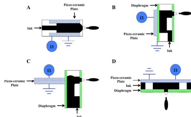
Fig. 5 Drop-on-demand piezoelectric inkjet printer. The piezoelectric inkjet printer applies a piezo-ceramic plate to create ink droplets. A thin diaphragm is bonded to the piezo-ceramic plate to prevent unintended interactions between the inks and the plate. The piezo-ceramic plate deforms in response to an electric impulse to generate a pressure wave to eject the ink. The ink is replenished on the removal of the electric pulse. At the same time, the piezo-ceramic plate returns to its normal shape. A: squeeze mode; B: bend mode; C: push mode; D: shear mode.
