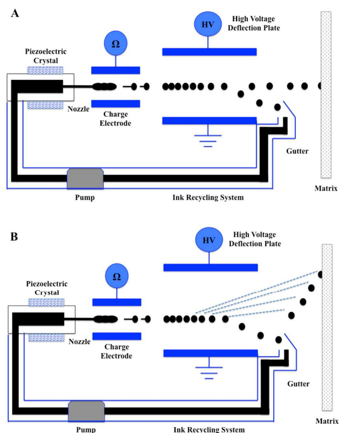
Fig. 3 Continuous inkjet printer systems. Ink droplets are constantly ejected, and the ejection is pumped by a piezoelectric crystal. The ink droplets are selectively charged via the printing signals. The charged droplets are deflected into a gutter for recirculation when passing through an electric field, while the uncharged droplets are ejected onto the matrix to form an image. A: In a binary deflection system, the uncharged droplets are printed onto the matrix and a single nozzle can only print at one dot position; B: In a multiple deflection system, the charged droplets are deflected onto the matrix. Multiple dots are deposited per nozzle.
