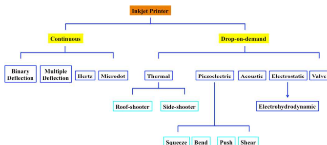
Fig. 2 Categories of inkjet printers.
