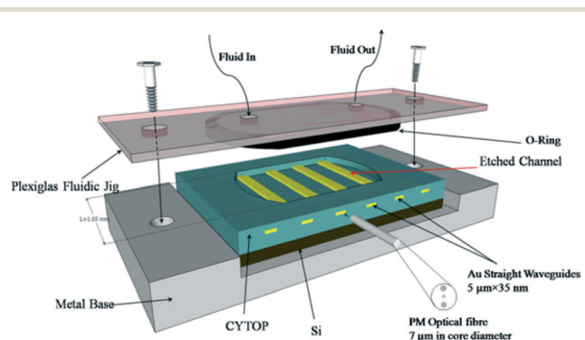
Fig. 1 Schematic representation of the sensor on the metal base with fluidic jig; the volume of the fluidic cell is 20\text{ }\mu\text{L} (adapted from ref. 22).
