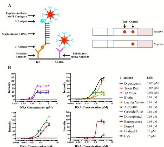
Fig. 1 (A). Design of single-plex LFDs: a dual-labeled analyte (RVFV DNA) was sandwiched between capture and detection antibodies due to antigen-antibody binding; AuNPs conjugated to the capture antibody (mouse anti-fluorescein antibody) enabled visualization of binding through the appearance of a red color at the test dot; rabbit anti-mouse antibody, which can directly bind the capture antibody (mouse anti-fluorescein), was deposited in parallel as a control. (B) Determination of detection limits for each single-plex assay: detection antibodies corresponding to the 3' antigen of dual-labeled RVFV were deposited at the test dot; resultant assay color intensity (average and standard deviation of 4 individual tests) was quantified using ImageJ software and plotted against DNA concentration; a cut-off defined as three standard deviations above the average was used to determine the limit of detection for each assay. Experimental details are described in the Supporting Information.
