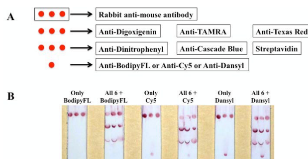
Fig. 2 Hepta-plex lateral flow detection results for combinations of seven antigen-antibody pairs. A: Positioning of detection antibodies deposited upon lateral flow strips. B: Hepta-plex lateral flow detection of 1 μM dual-labeled analyte alone (containing either 3' BodipyFL, Cy5, or Dansyl), or combinations of dual-labeled analyte (1 μM) containing 3' Biotin, Cascade Blue, Digoxigenin, Dinitrophenyl, TAMRA, and Texas Red and either BodipyFL, Cy5 or Dansyl, as indicated. Assay was repeated three times and a representative photograph is shown. Experimental details are described in the Supporting Information.
