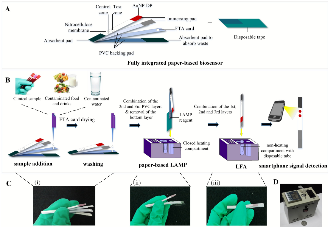
Figure 1. Schematic of an integrated paper-based sample-to-answer biosensor. (A) The integrated paper-based biosensor composed of four hydrophobic polyvinyl chloride (PVC) layers to control the sample flow from nucleic acid extraction zone to amplification zone and lateral flow strip. (B) The schematic diagram of experimental procedure. (C) The photo images of the biosensor during the steps of (i) extraction, (ii) amplification and (iii) lateral flow detection. (D) The photo images of a handheld heating device.
