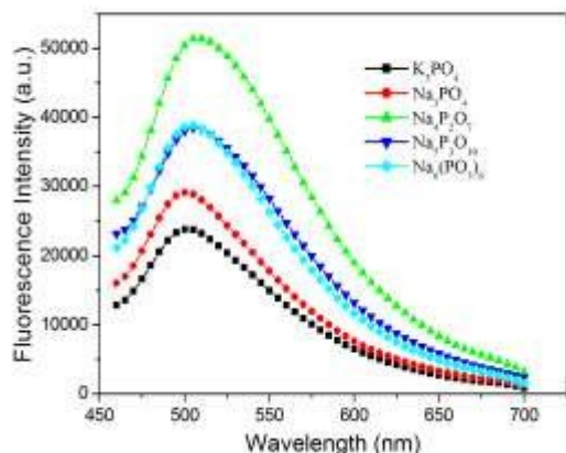
Fig.1 Fluorescence emission spectra of CDs excited at 420 nm respectively prepared with potassium phosphate (125 mmol/L), sodium phosphate (125 mmol/L), sodium pyrophosphate (62.5 mmol/L), sodium triphosphate (41.7 mmol/L) or sodium hexametaphosphate (20.8 mmol/L).
