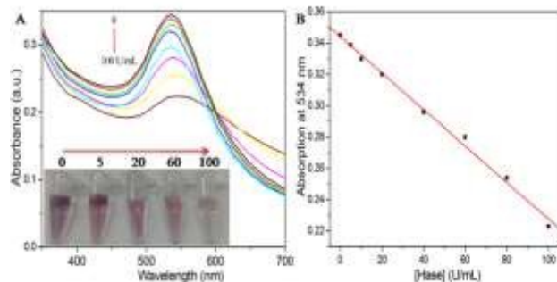
Fig.5 (A) UV-Vis absorption spectra of CDs/HA-Au NPs SET system incubated with different concentrations of Hase (0, 5, 10, 20, 40, 60, 80, 100 U/mL) for 2 hours. The inset picture shows the color change of the SET system solutions incubated with different concentrations of Hase (0, 5, 20, 60, 100 U/mL) for 2 hours. (B) The standard curve of absorbance at 534 nm as the function of Hase concentration (0, 5, 10, 20, 40, 60, 80, 100 U/mL).
