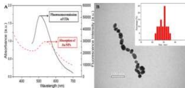
Fig.3 (A) The fluorescence emission spectra of CDs (solid line) and UV-Vis absorption spectra of HA-Au NPs solution (dashed line). (B) The TEM image of HA-Au NPs.
